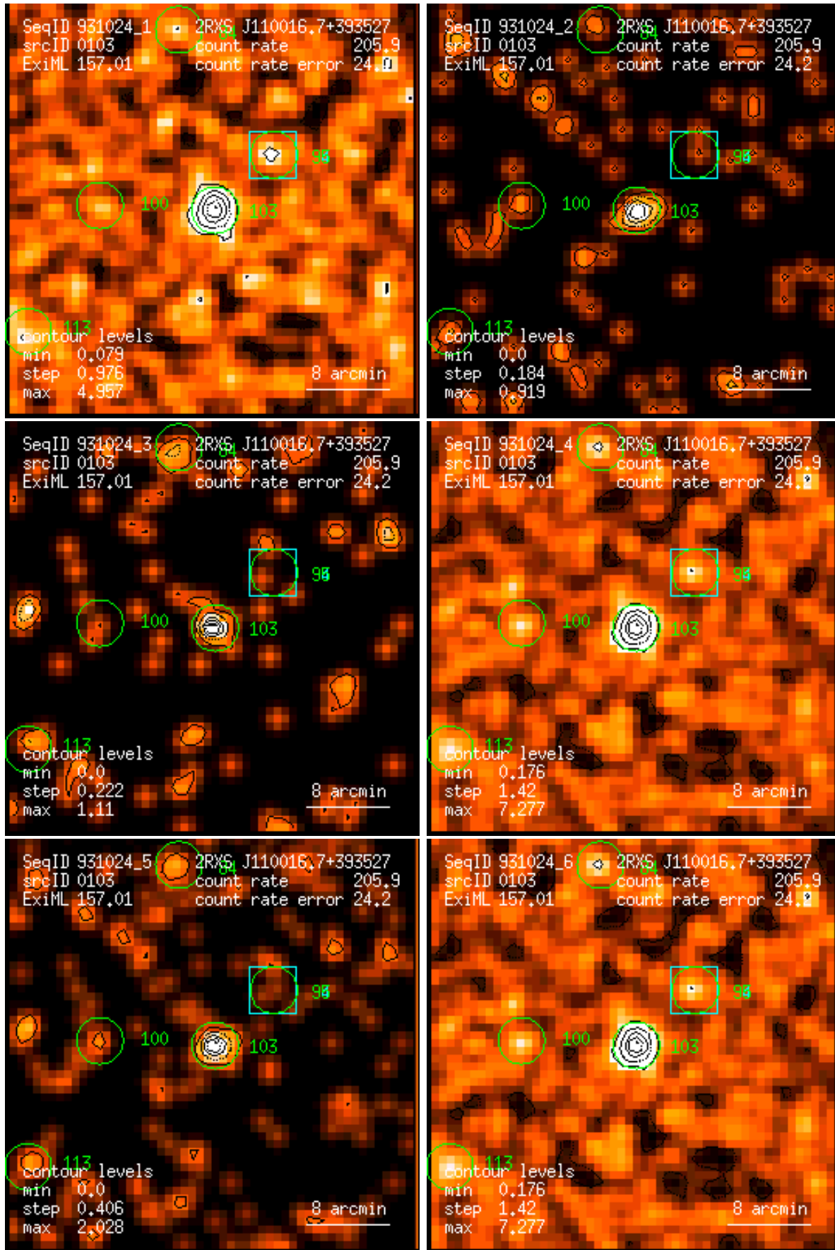
Figure 103: RASS 931024: detection 0103: band rate images, Gaussian filter: (1) PSPC channels 11 – 41, (2) 52 – 90, (3) 91 – 201, (4) 11 – 235, (5) 52 – 201, (6) 11 – 201. Broad band rates in counts/ks. Band rate contour levels in counts/ks/arcmin 2 .
