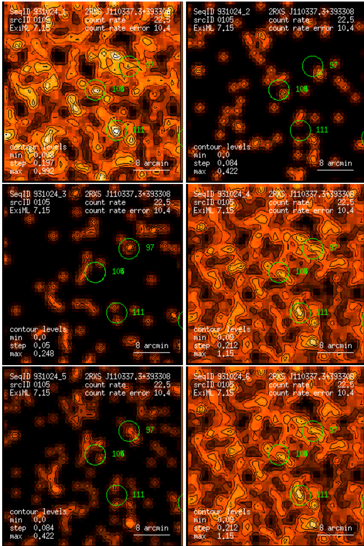
Figure 105: RASS 931024: detection 0105: band rate images, Gaussian filter: (1) PSPC channels 11 – 41, (2) 52 – 90, (3) 91 – 201, (4) 11 – 235, (5) 52 – 201, (6) 11 – 201. Broad band rates in counts/ks. Band rate contour levels in counts/ks/arcmin 2 .
