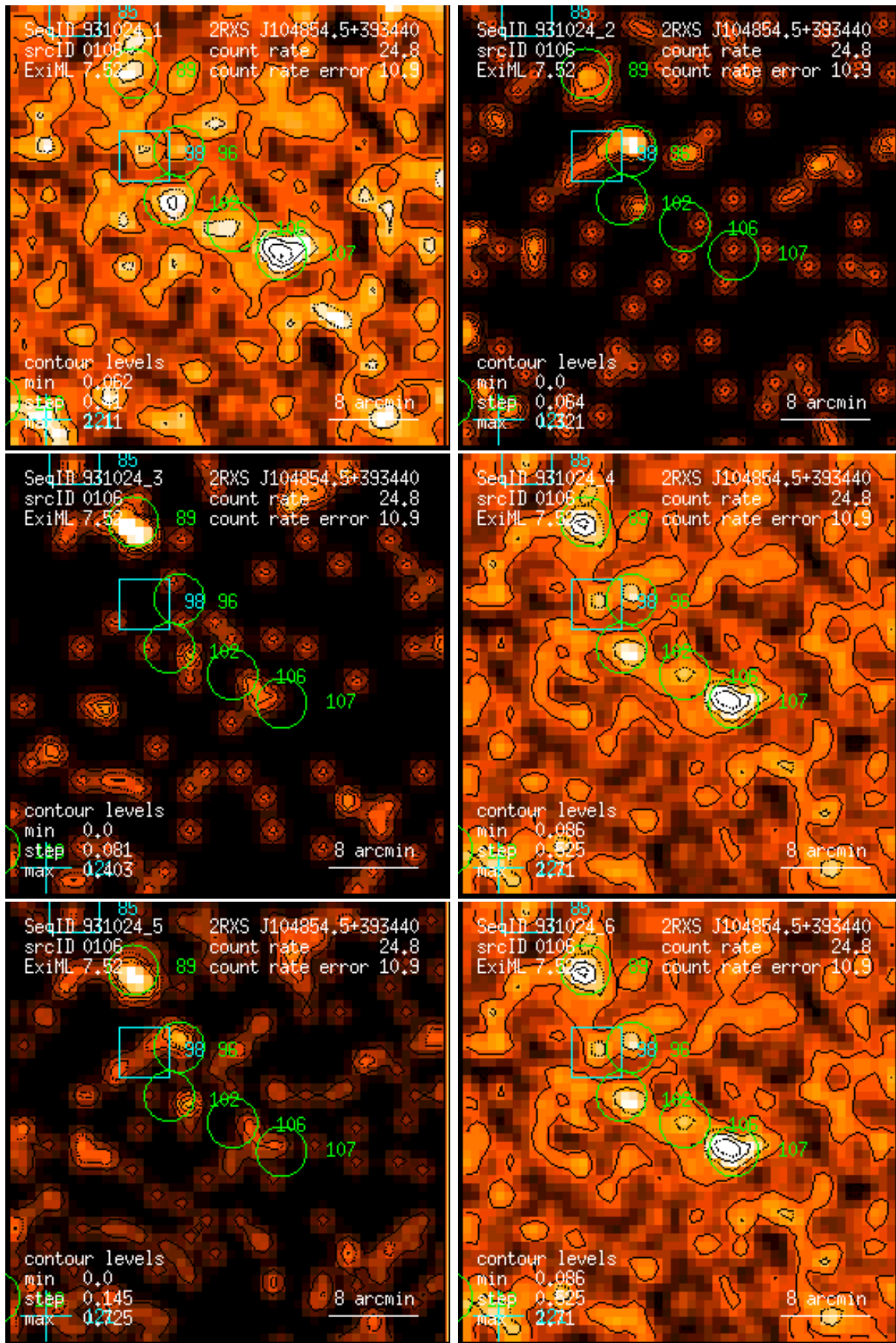
Figure 106: RASS 931024: detection 0106: band rate images, Gaussian filter: (1) PSPC channels 11 – 41, (2) 52 – 90, (3) 91 – 201, (4) 11 – 235, (5) 52 – 201, (6) 11 – 201. Broad band rates in counts/ks. Band rate contour levels in counts/ks/arcmin 2 .
