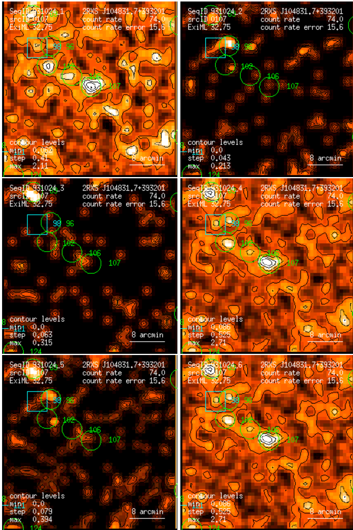
Figure 107: RASS 931024: detection 0107: band rate images, Gaussian filter: (1) PSPC channels 11 – 41, (2) 52 – 90, (3) 91 – 201, (4) 11 – 235, (5) 52 – 201, (6) 11 – 201. Broad band rates in counts/ks. Band rate contour levels in counts/ks/arcmin 2 .
