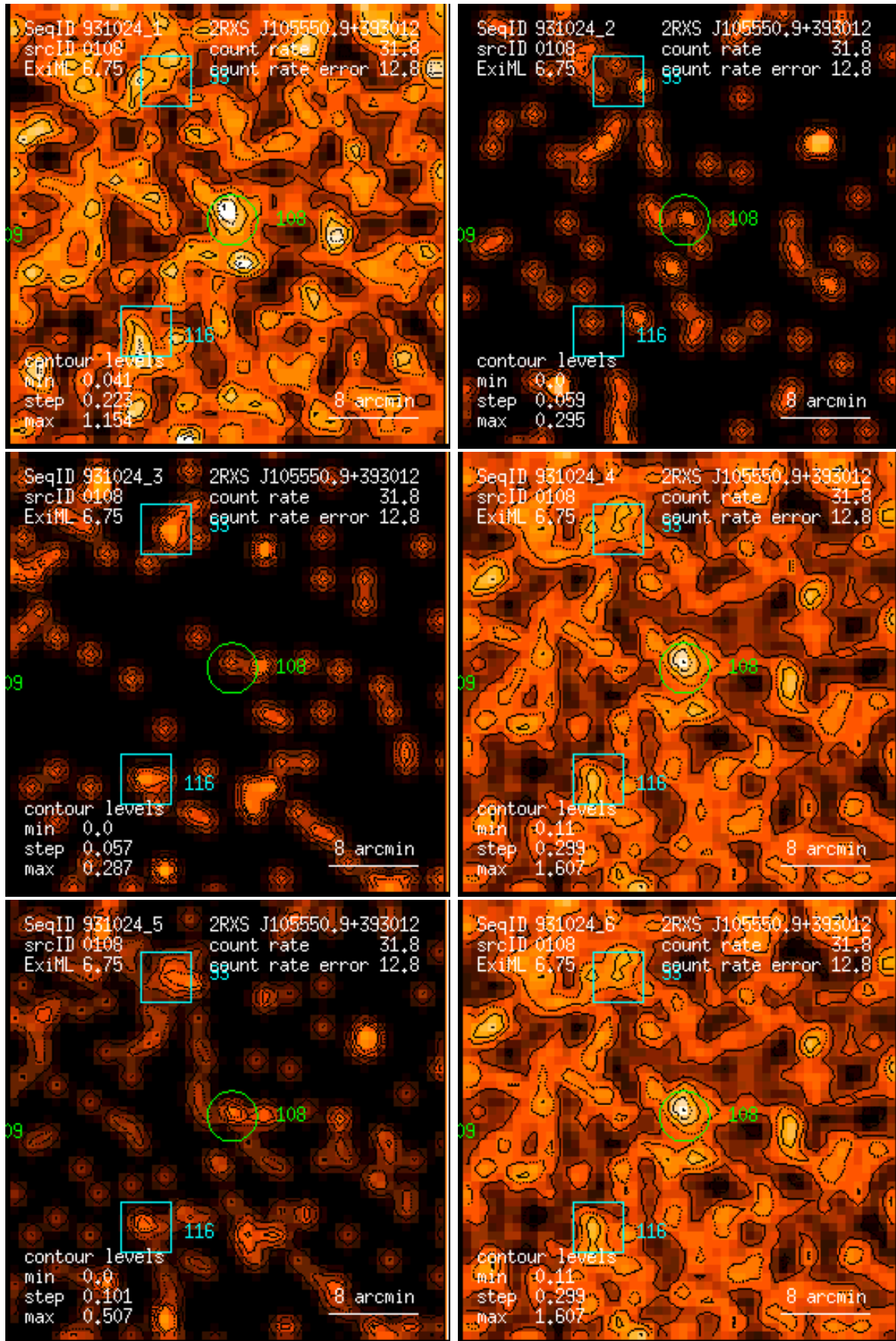
Figure 108: RASS 931024: detection 0108: band rate images, Gaussian filter: (1) PSPC channels 11 – 41, (2) 52 – 90, (3) 91 – 201, (4) 11 – 235, (5) 52 – 201, (6) 11 – 201. Broad band rates in counts/ks. Band rate contour levels in counts/ks/arcmin 2 .
