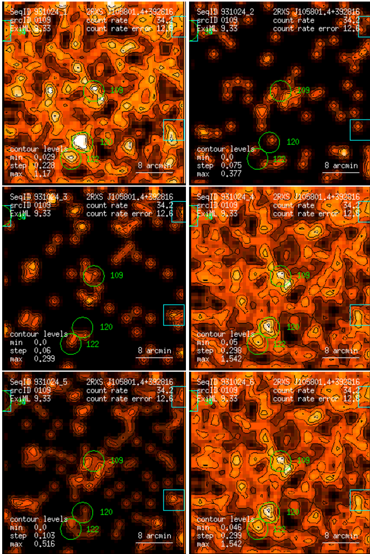
Figure 109: RASS 931024: detection 0109: band rate images, Gaussian filter: (1) PSPC channels 11 – 41, (2) 52 – 90, (3) 91 – 201, (4) 11 – 235, (5) 52 – 201, (6) 11 – 201. Broad band rates in counts/ks. Band rate contour levels in counts/ks/arcmin 2 .
