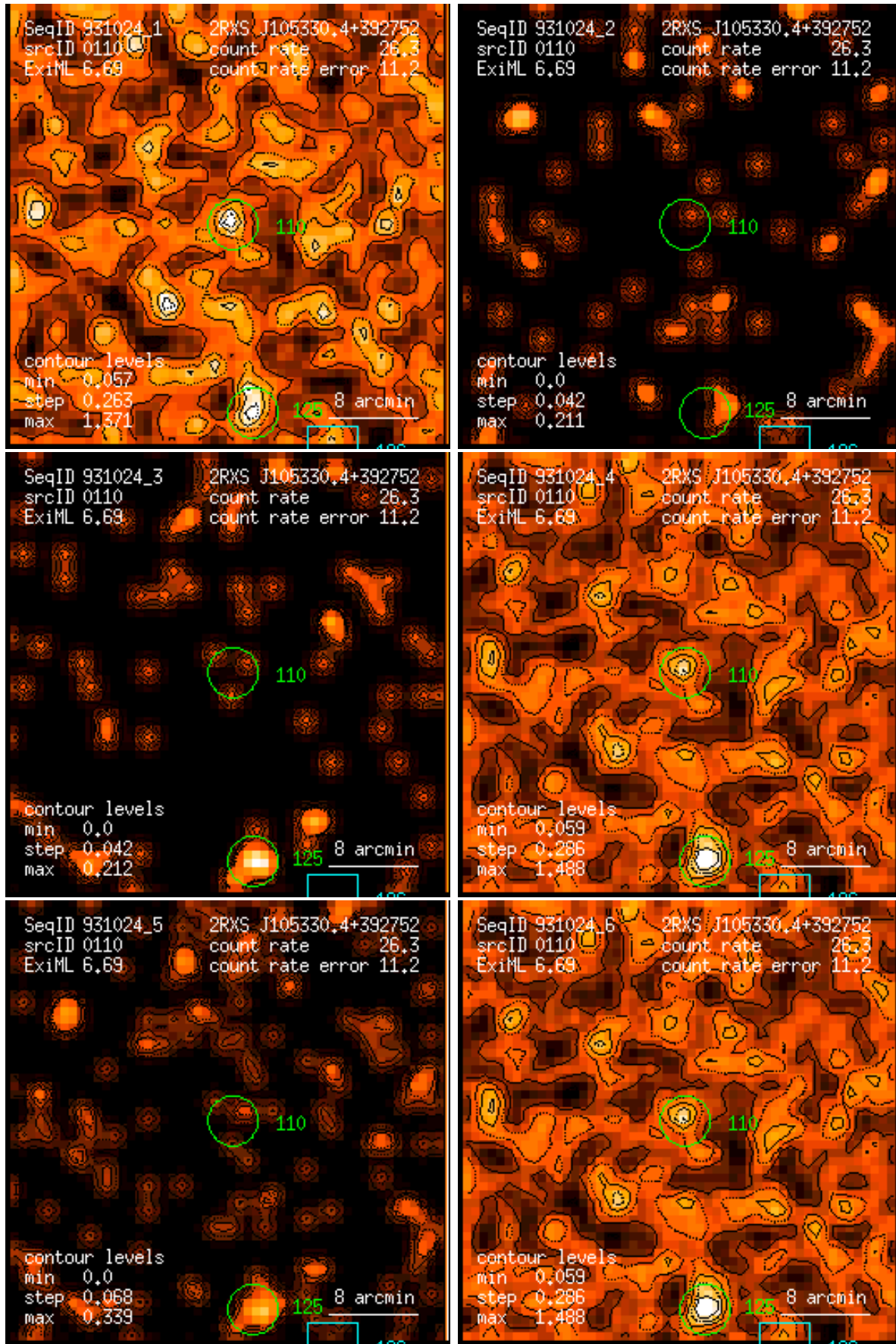
Figure 110: RASS 931024: detection 0110: band rate images, Gaussian filter: (1) PSPC channels 11 – 41, (2) 52 – 90, (3) 91 – 201, (4) 11 – 235, (5) 52 – 201, (6) 11 – 201. Broad band rates in counts/ks. Band rate contour levels in counts/ks/arcmin 2 .
