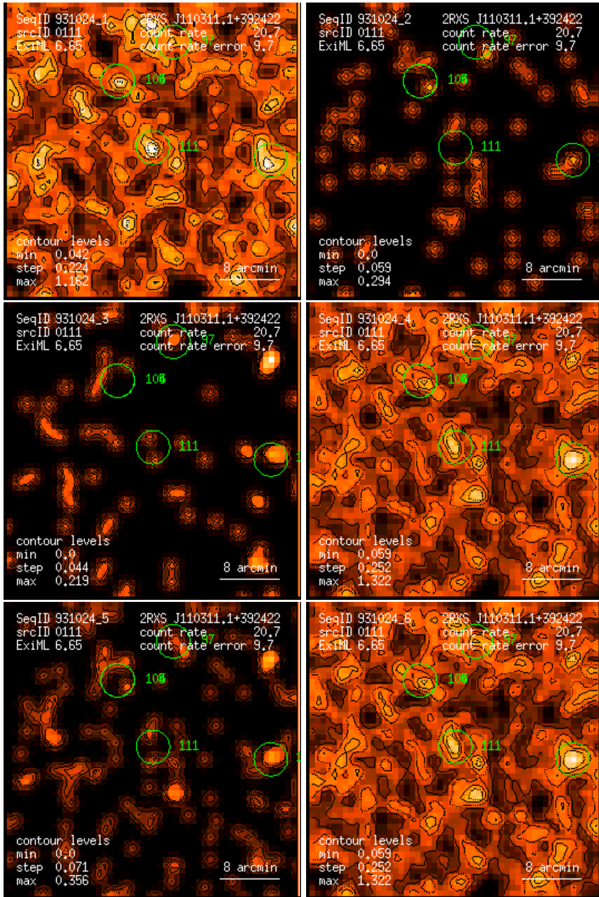
Figure 111: RASS 931024: detection 0111: band rate images, Gaussian filter: (1) PSPC channels 11 – 41, (2) 52 – 90, (3) 91 – 201, (4) 11 – 235, (5) 52 – 201, (6) 11 – 201. Broad band rates in counts/ks. Band rate contour levels in counts/ks/arcmin 2 .
