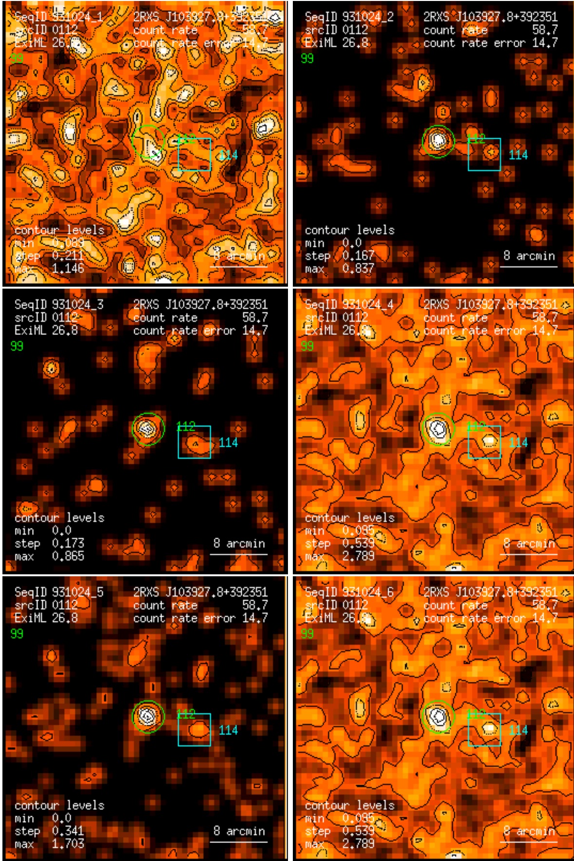
Figure 112: RASS 931024: detection 0112: band rate images, Gaussian filter: (1) PSPC channels 11 – 41, (2) 52 – 90, (3) 91 – 201, (4) 11 – 235, (5) 52 – 201, (6) 11 – 201. Broad band rates in counts/ks. Band rate contour levels in counts/ks/arcmin 2 .
