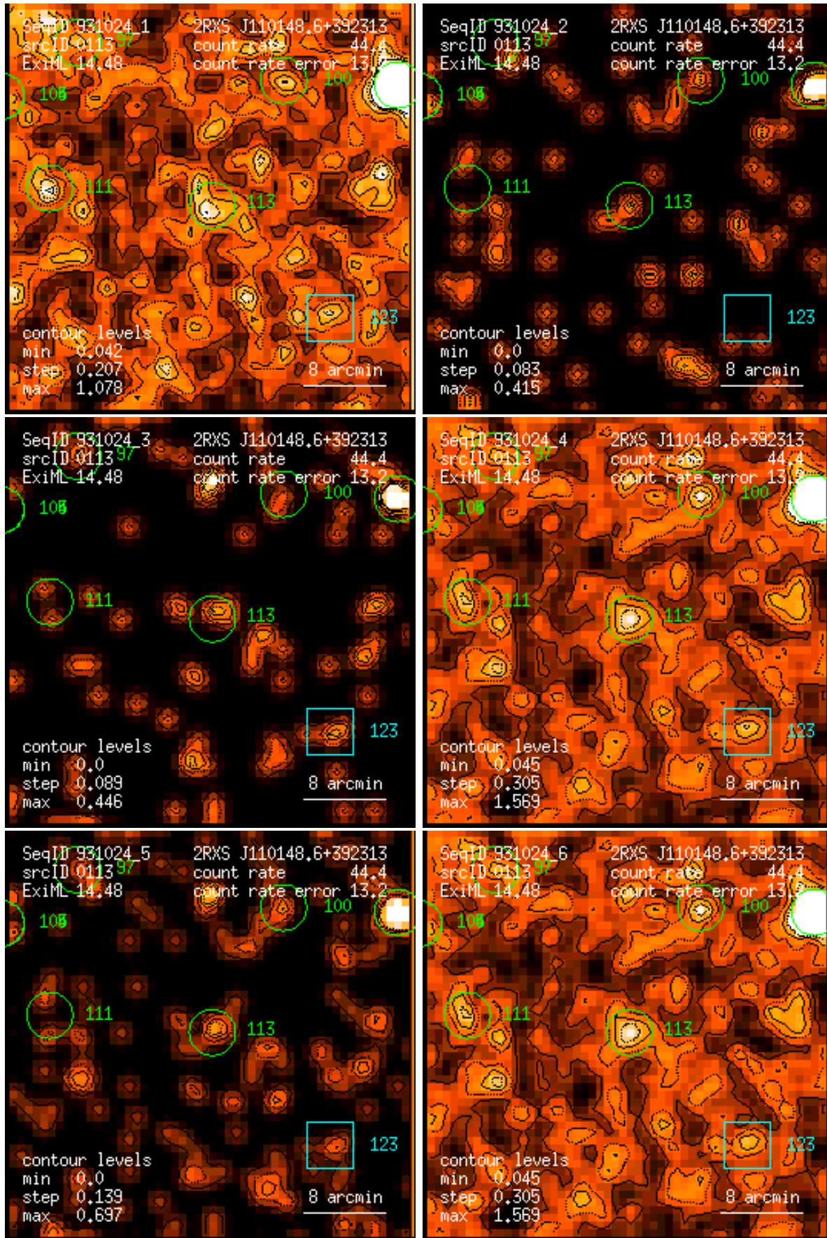
Figure 113: RASS 931024: detection 0113: band rate images, Gaussian filter: (1) PSPC channels 11 – 41, (2) 52 – 90, (3) 91 – 201, (4) 11 – 235, (5) 52 – 201, (6) 11 – 201. Broad band rates in counts/ks. Band rate contour levels in counts/ks/arcmin 2 .
