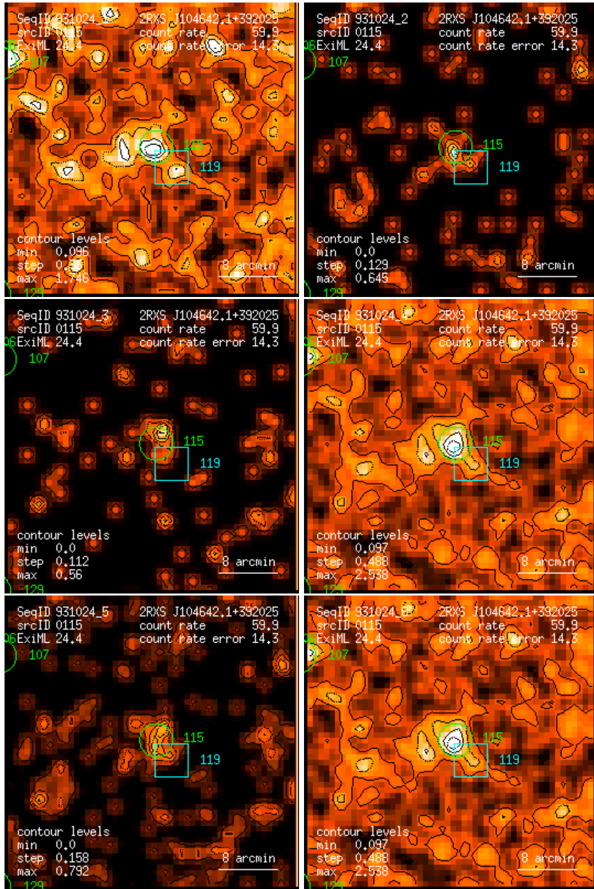
Figure 115: RASS 931024: detection 0115: band rate images, Gaussian filter: (1) PSPC channels 11 – 41, (2) 52 – 90, (3) 91 – 201, (4) 11 – 235, (5) 52 – 201, (6) 11 – 201. Broad band rates in counts/ks. Band rate contour levels in counts/ks/arcmin 2 .
