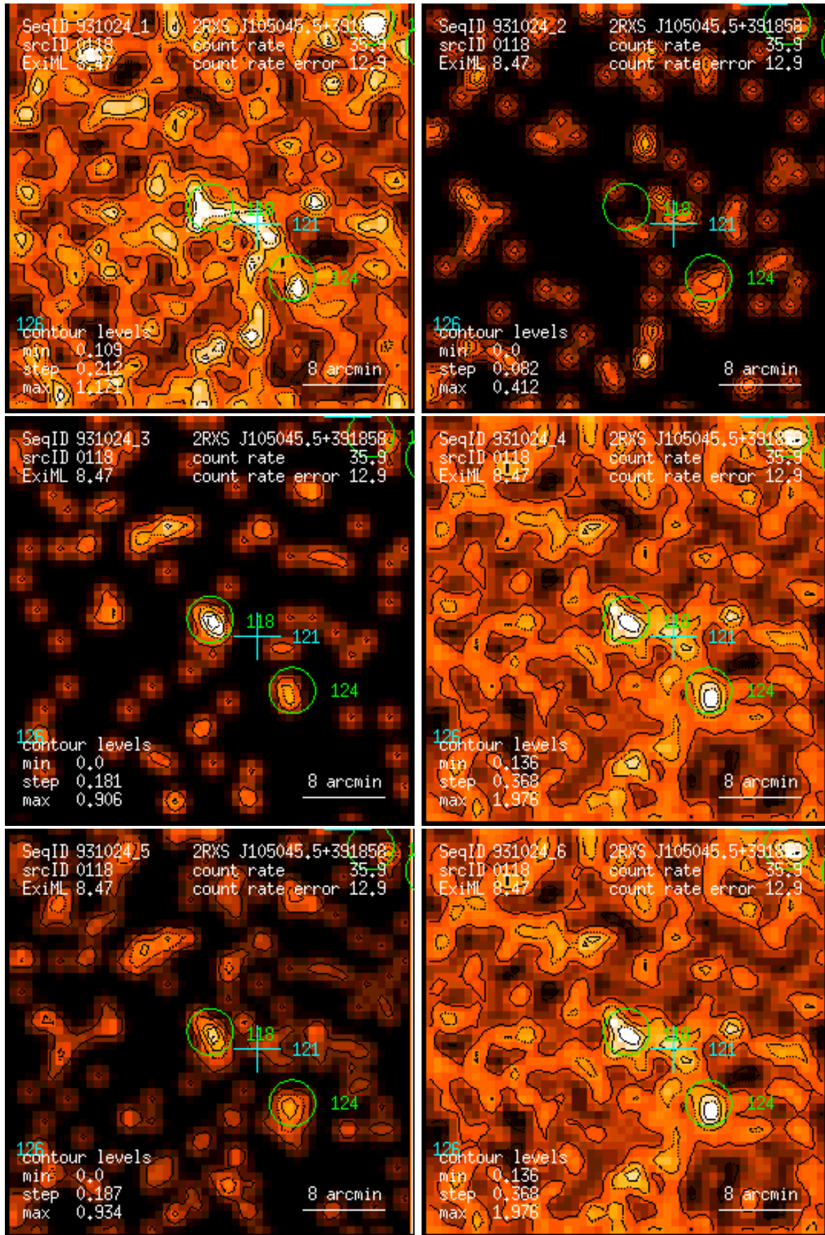
Figure 118: RASS 931024: detection 0118: band rate images, Gaussian filter: (1) PSPC channels 11 – 41, (2) 52 – 90, (3) 91 – 201, (4) 11 – 235, (5) 52 – 201, (6) 11 – 201. Broad band rates in counts/ks. Band rate contour levels in counts/ks/arcmin 2 .
