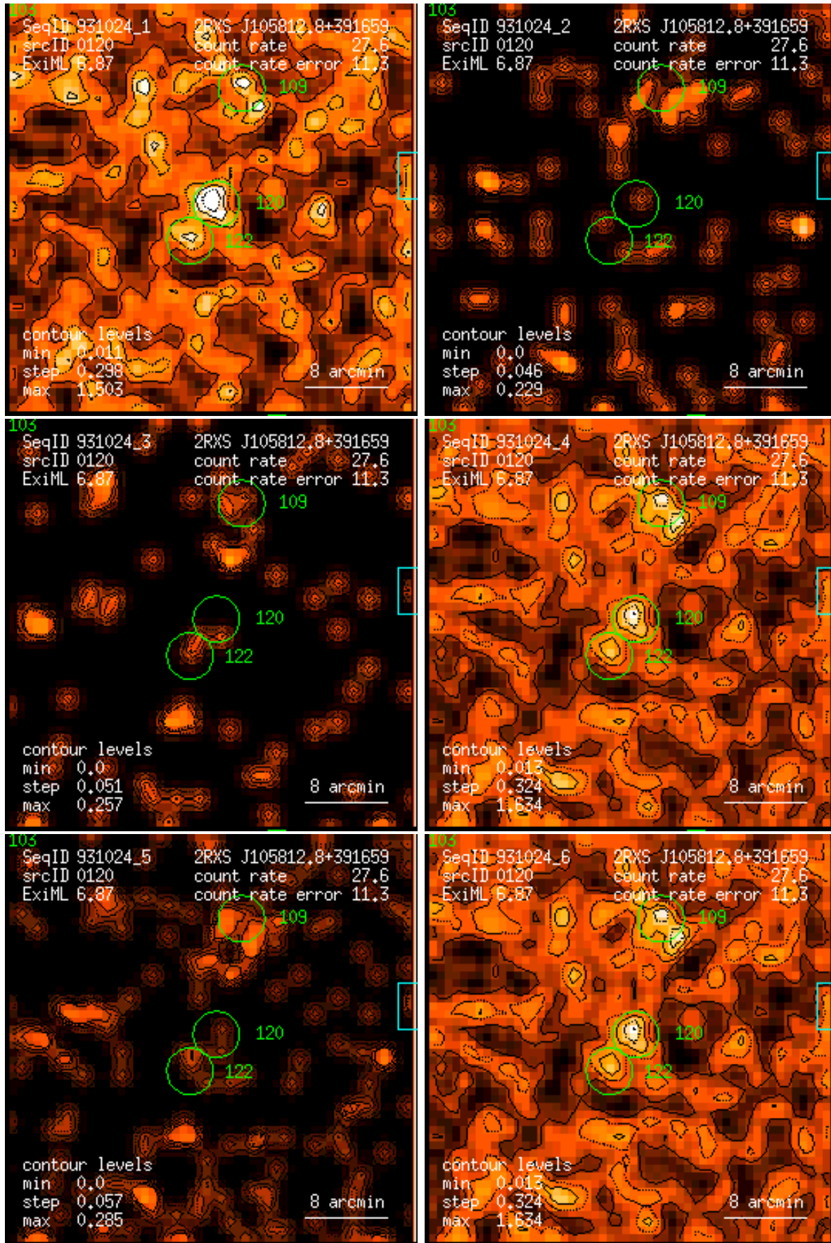
Figure 120: RASS 931024: detection 0120: band rate images, Gaussian filter: (1) PSPC channels 11 – 41, (2) 52 – 90, (3) 91 – 201, (4) 11 – 235, (5) 52 – 201, (6) 11 – 201. Broad band rates in counts/ks. Band rate contour levels in counts/ks/arcmin 2 .
