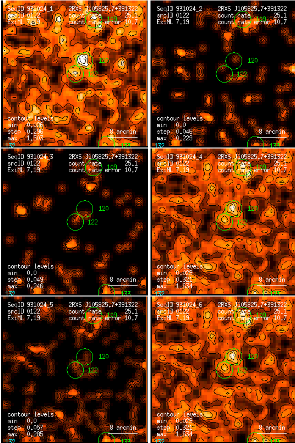
Figure 122: RASS 931024: detection 0122: band rate images, Gaussian filter: (1) PSPC channels 11 – 41, (2) 52 – 90, (3) 91 – 201, (4) 11 – 235, (5) 52 – 201, (6) 11 – 201. Broad band rates in counts/ks. Band rate contour levels in counts/ks/arcmin 2 .
