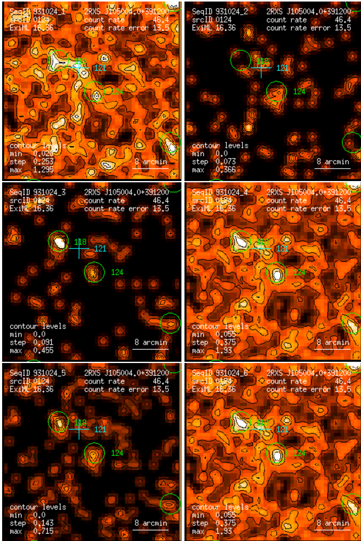
Figure 124: RASS 931024: detection 0124: band rate images, Gaussian filter: (1) PSPC channels 11 – 41, (2) 52 – 90, (3) 91 – 201, (4) 11 – 235, (5) 52 – 201, (6) 11 – 201. Broad band rates in counts/ks. Band rate contour levels in counts/ks/arcmin 2 .
