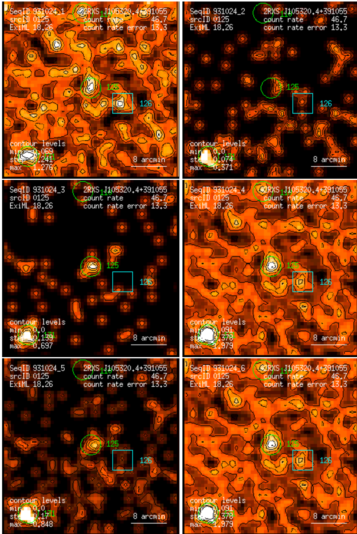
Figure 125: RASS 931024: detection 0125: band rate images, Gaussian filter: (1) PSPC channels 11 – 41, (2) 52 – 90, (3) 91 – 201, (4) 11 – 235, (5) 52 – 201, (6) 11 – 201. Broad band rates in counts/ks. Band rate contour levels in counts/ks/arcmin 2 .
