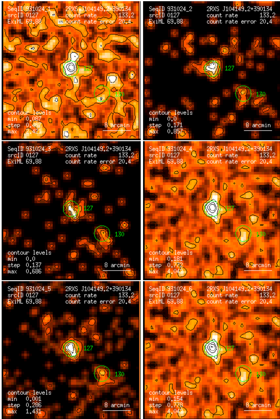
Figure 127: RASS 931024: detection 0127: band rate images, Gaussian filter: (1) PSPC channels 11 – 41, (2) 52 – 90, (3) 91 – 201, (4) 11 – 235, (5) 52 – 201, (6) 11 – 201. Broad band rates in counts/ks. Band rate contour levels in counts/ks/arcmin 2 .
