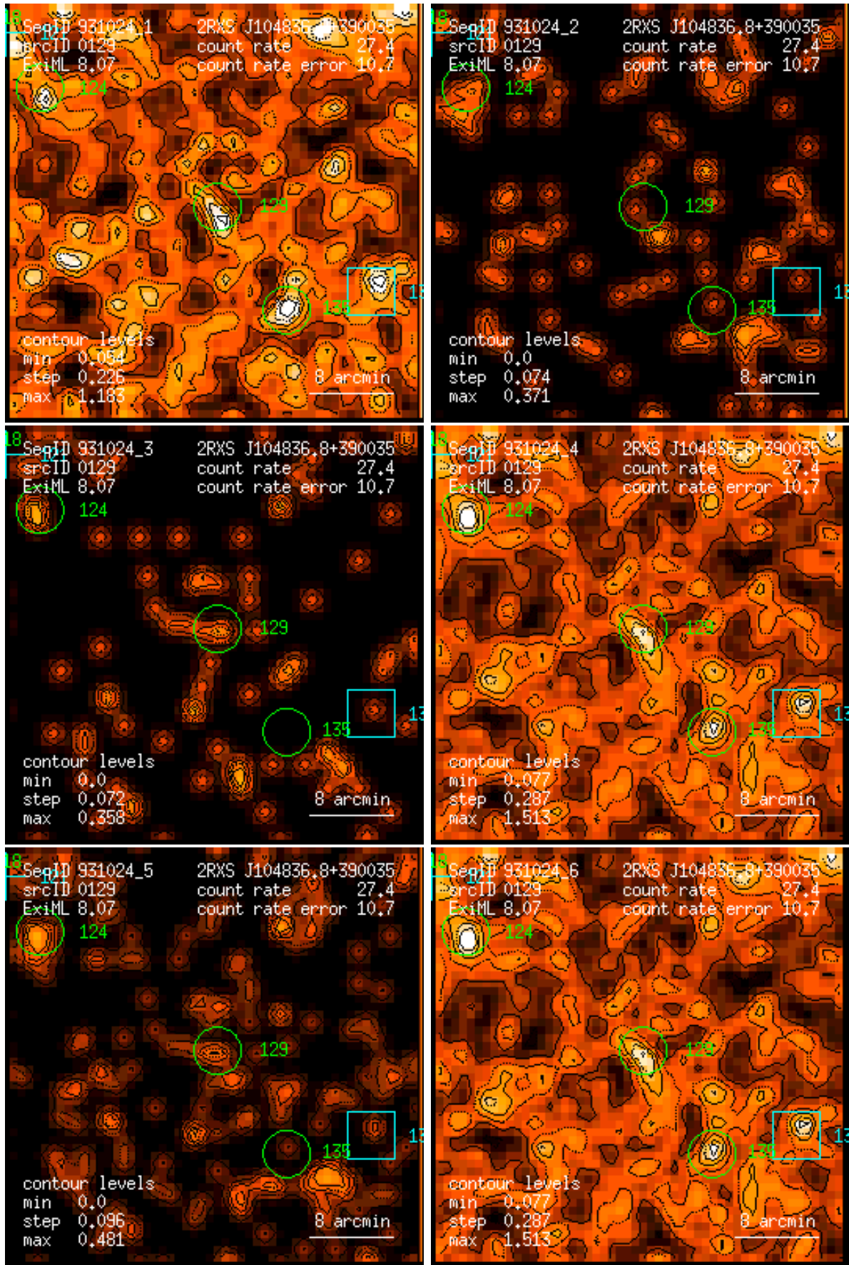
Figure 129: RASS 931024: detection 0129: band rate images, Gaussian filter: (1) PSPC channels 11 – 41, (2) 52 – 90, (3) 91 – 201, (4) 11 – 235, (5) 52 – 201, (6) 11 – 201. Broad band rates in counts/ks. Band rate contour levels in counts/ks/arcmin 2 .
