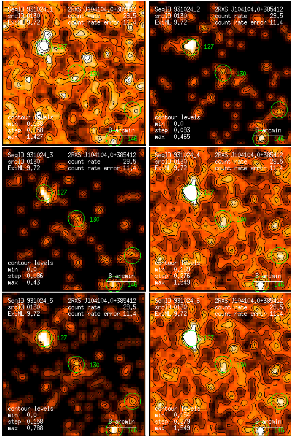
Figure 130: RASS 931024: detection 0130: band rate images, Gaussian filter: (1) PSPC channels 11 – 41, (2) 52 – 90, (3) 91 – 201, (4) 11 – 235, (5) 52 – 201, (6) 11 – 201. Broad band rates in counts/ks. Band rate contour levels in counts/ks/arcmin 2 .
