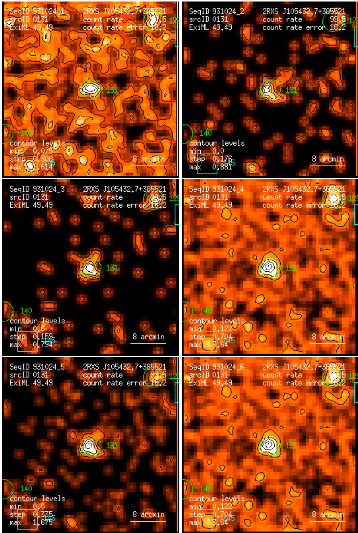
Figure 131: RASS 931024: detection 0131: band rate images, Gaussian filter: (1) PSPC channels 11 – 41, (2) 52 – 90, (3) 91 – 201, (4) 11 – 235, (5) 52 – 201, (6) 11 – 201. Broad band rates in counts/ks. Band rate contour levels in counts/ks/arcmin 2 .
