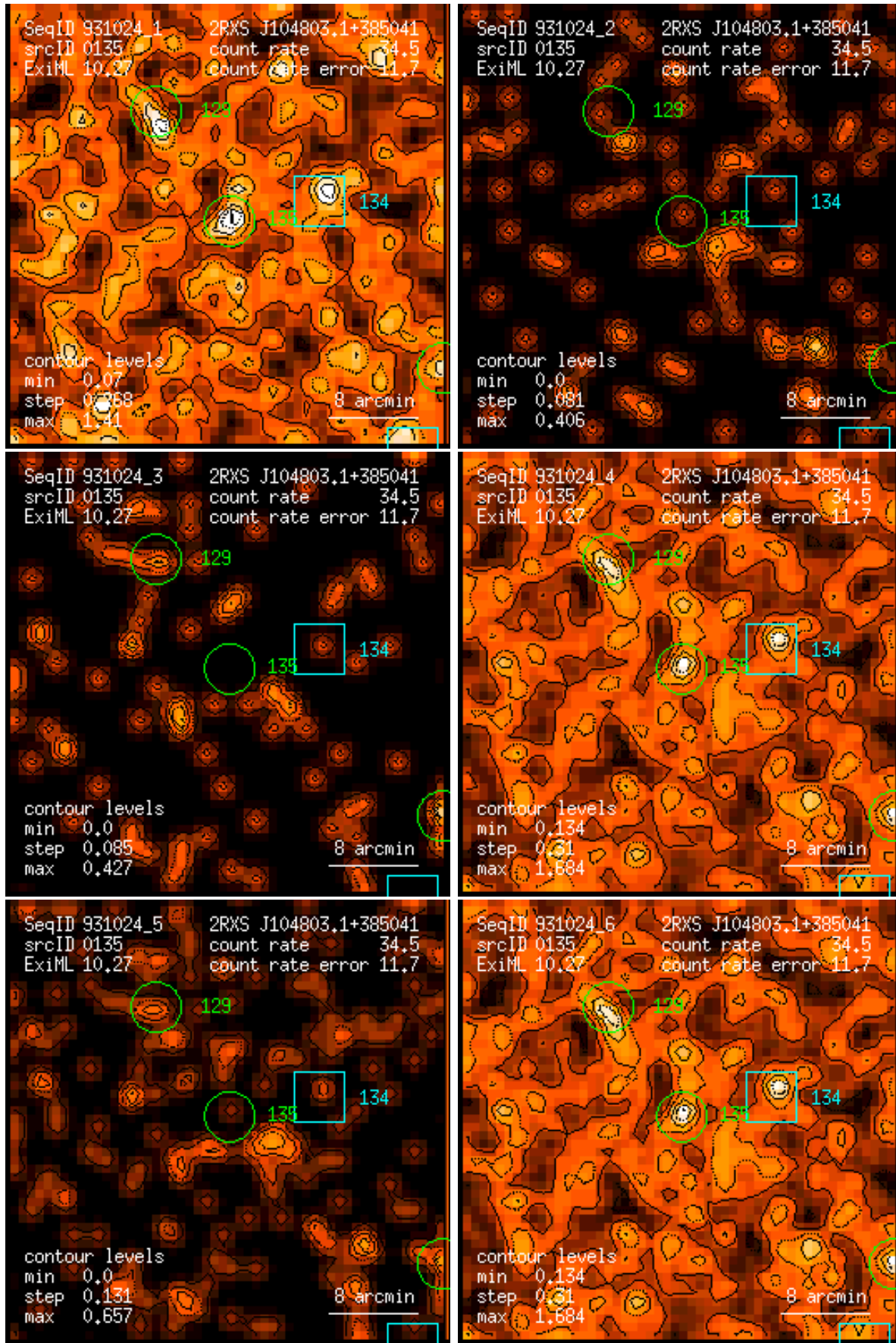
Figure 135: RASS 931024: detection 0135: band rate images, Gaussian filter: (1) PSPC channels 11 – 41, (2) 52 – 90, (3) 91 – 201, (4) 11 – 235, (5) 52 – 201, (6) 11 – 201. Broad band rates in counts/ks. Band rate contour levels in counts/ks/arcmin 2 .
