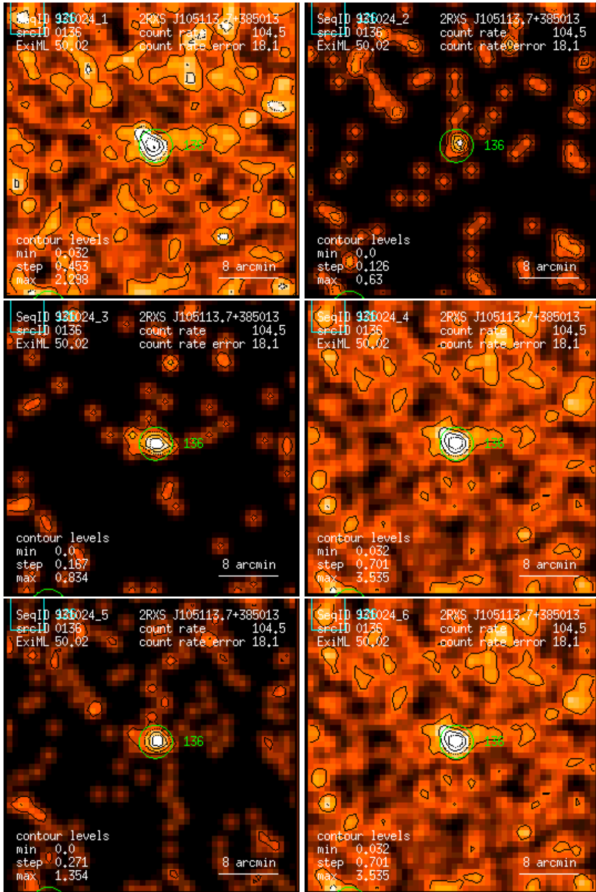
Figure 136: RASS 931024: detection 0136: band rate images, Gaussian filter: (1) PSPC channels 11 – 41, (2) 52 – 90, (3) 91 – 201, (4) 11 – 235, (5) 52 – 201, (6) 11 – 201. Broad band rates in counts/ks. Band rate contour levels in counts/ks/arcmin 2 .
