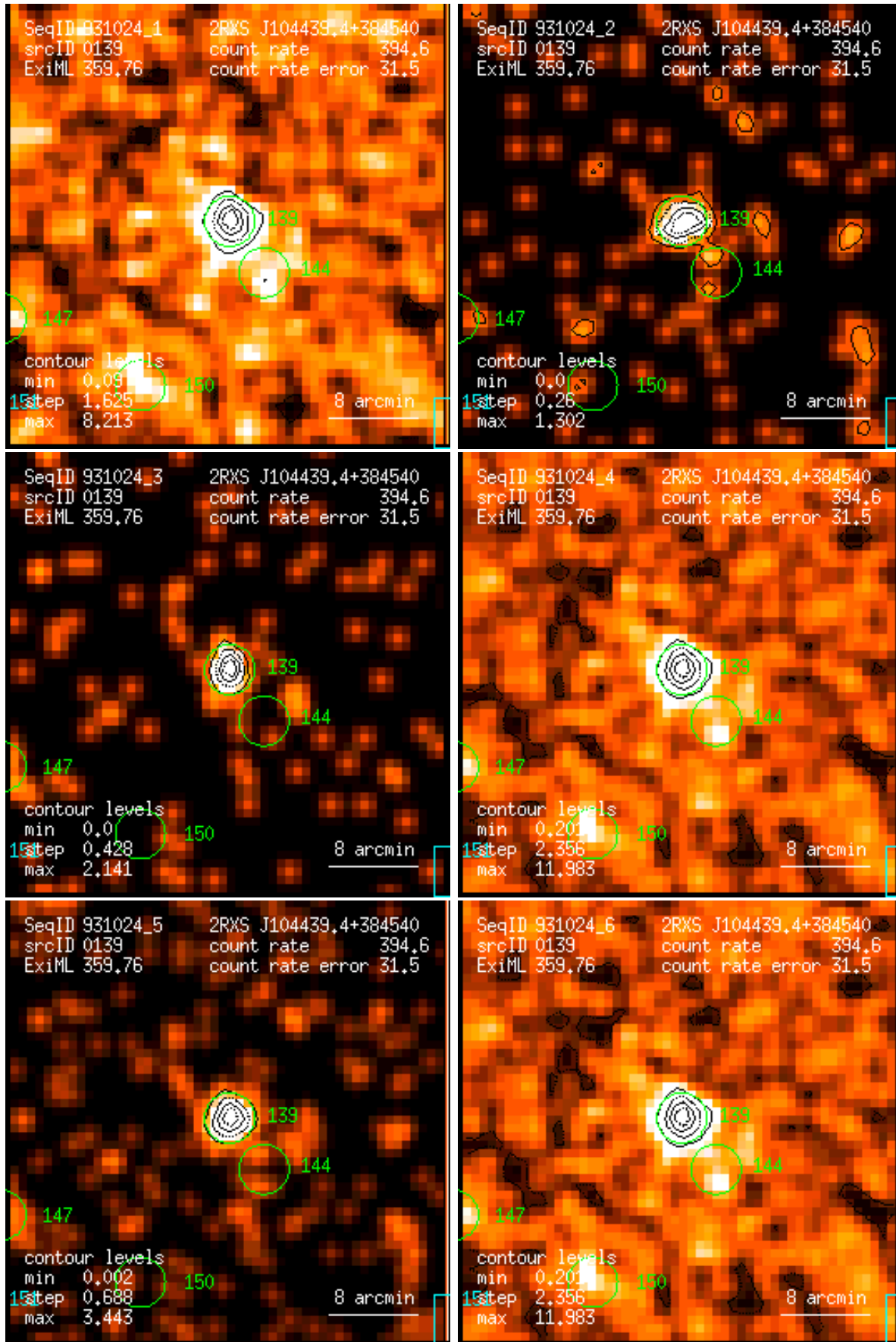
Figure 139: RASS 931024: detection 0139: band rate images, Gaussian filter: (1) PSPC channels 11 – 41, (2) 52 – 90, (3) 91 – 201, (4) 11 – 235, (5) 52 – 201, (6) 11 – 201. Broad band rates in counts/ks. Band rate contour levels in counts/ks/arcmin 2 .
