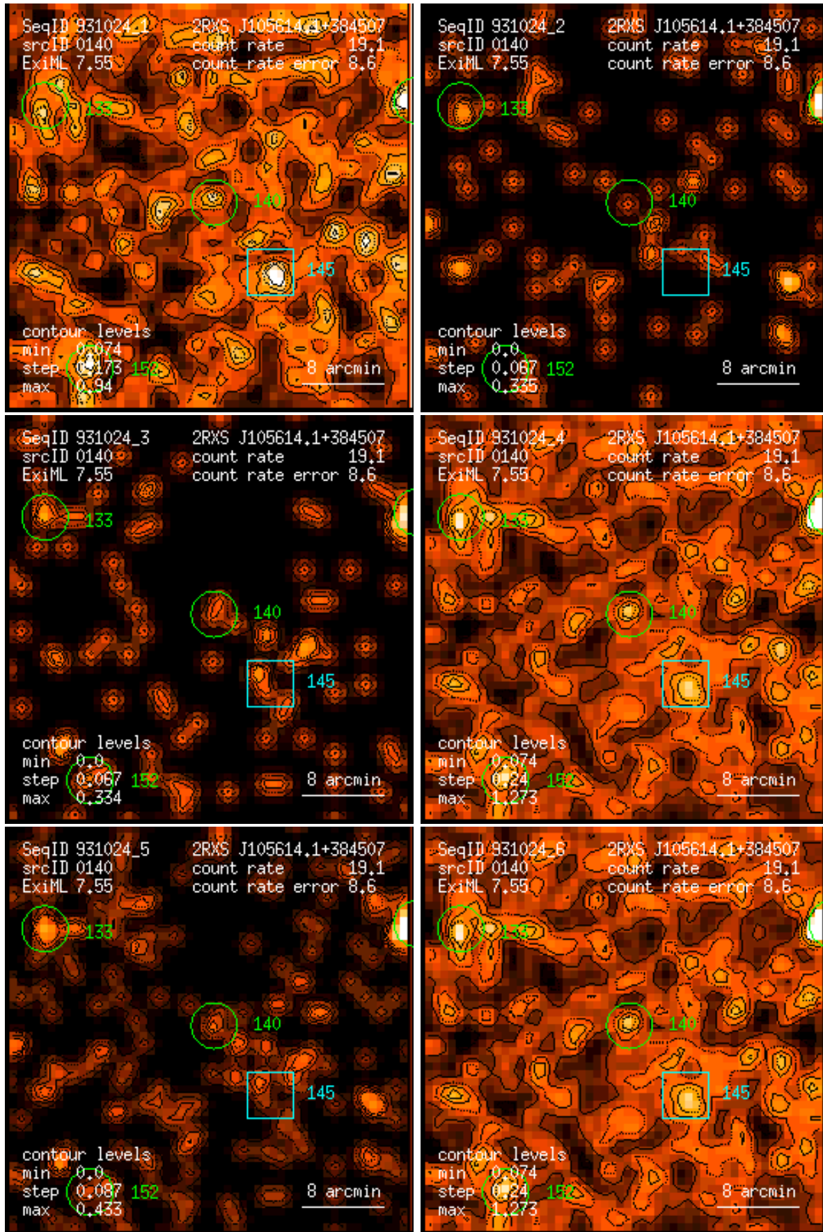
Figure 140: RASS 931024: detection 0140: band rate images, Gaussian filter: (1) PSPC channels 11 – 41, (2) 52 – 90, (3) 91 – 201, (4) 11 – 235, (5) 52 – 201, (6) 11 – 201. Broad band rates in counts/ks. Band rate contour levels in counts/ks/arcmin 2 .
