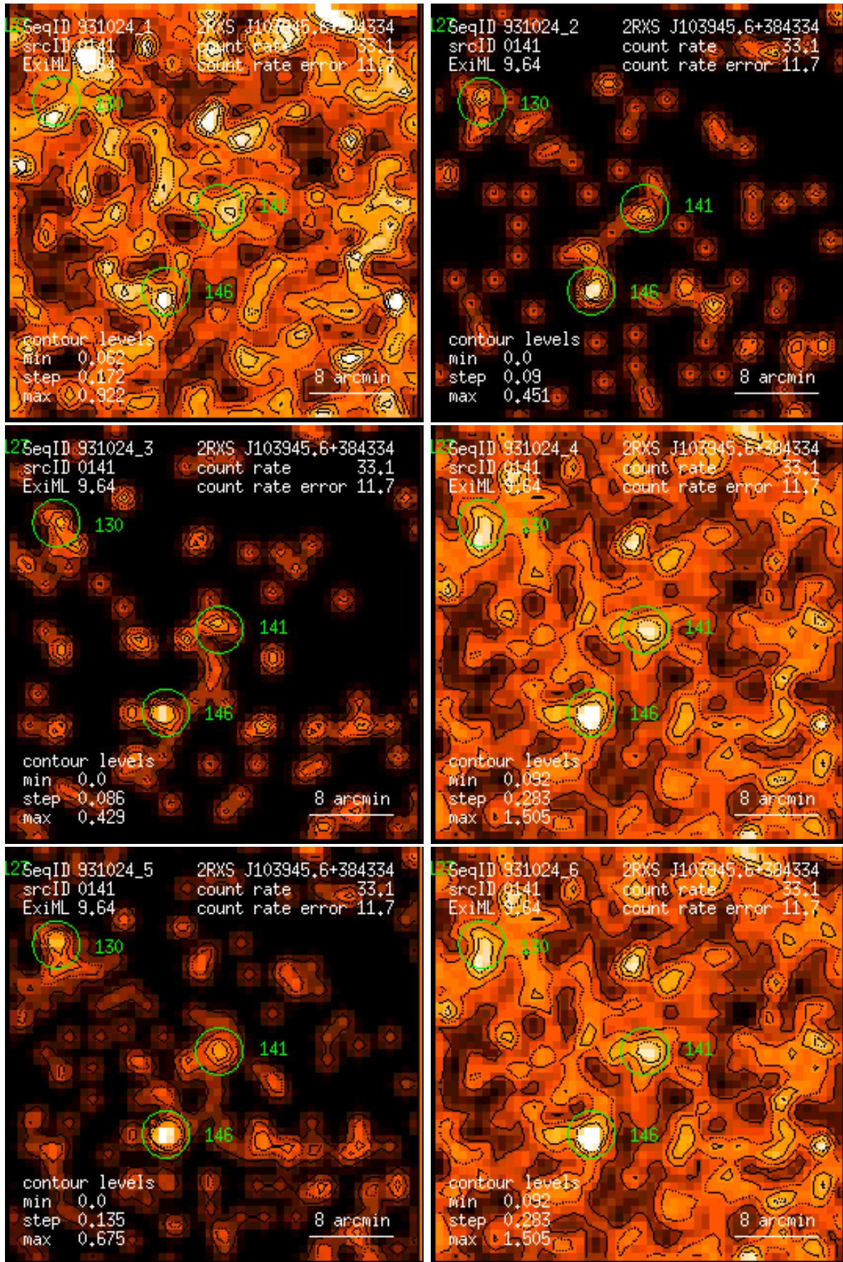
Figure 141: RASS 931024: detection 0141: band rate images, Gaussian filter: (1) PSPC channels 11 – 41, (2) 52 – 90, (3) 91 – 201, (4) 11 – 235, (5) 52 – 201, (6) 11 – 201. Broad band rates in counts/ks. Band rate contour levels in counts/ks/arcmin 2 .
