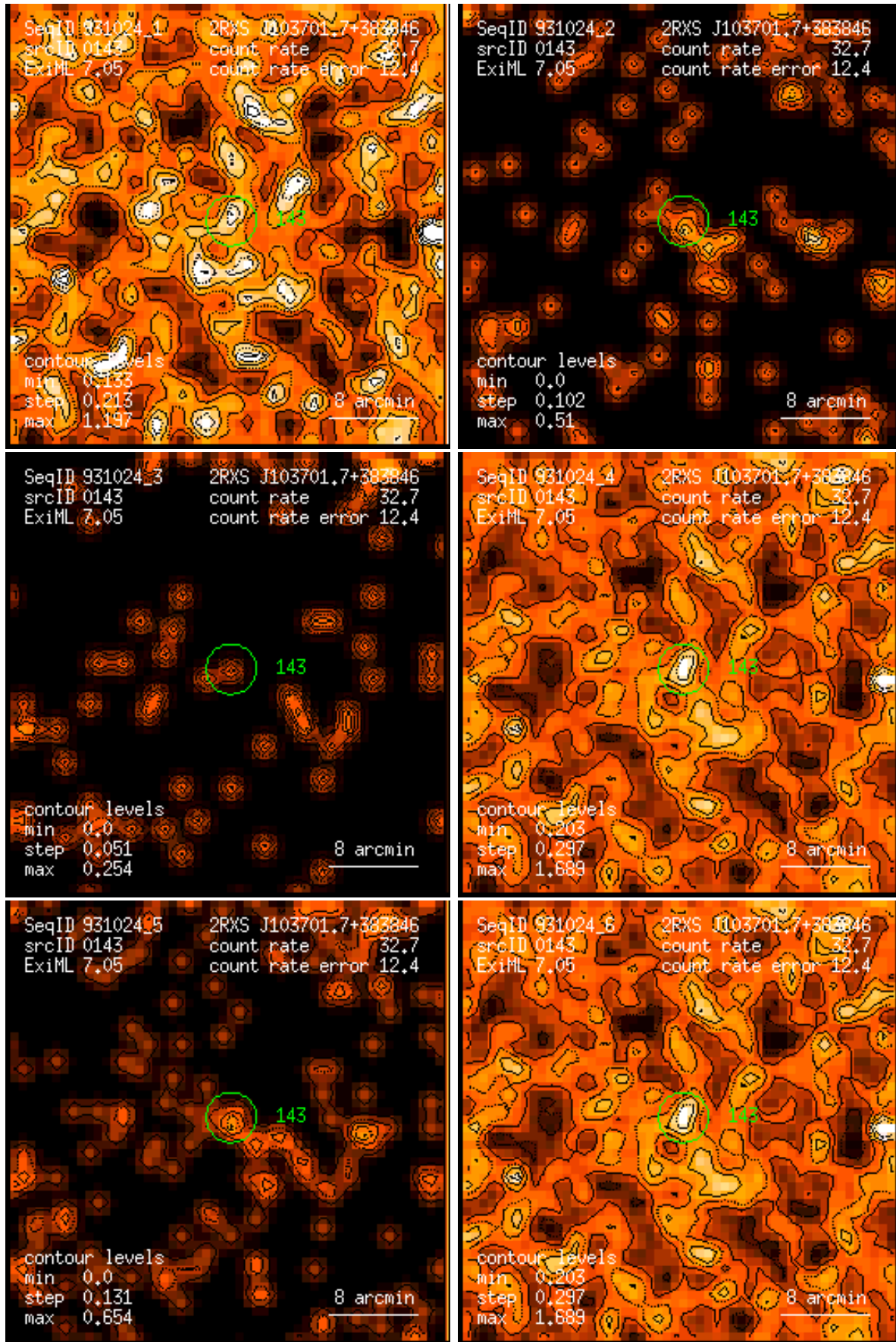
Figure 143: RASS 931024: detection 0143: band rate images, Gaussian filter: (1) PSPC channels 11 – 41, (2) 52 – 90, (3) 91 – 201, (4) 11 – 235, (5) 52 – 201, (6) 11 – 201. Broad band rates in counts/ks. Band rate contour levels in counts/ks/arcmin 2 .
