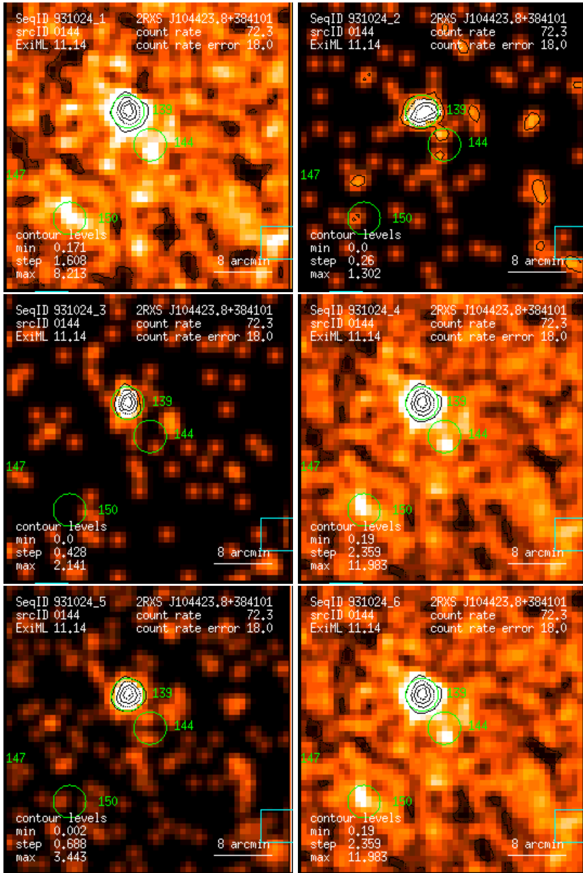
Figure 144: RASS 931024: detection 0144: band rate images, Gaussian filter: (1) PSPC channels 11 – 41, (2) 52 – 90, (3) 91 – 201, (4) 11 – 235, (5) 52 – 201, (6) 11 – 201. Broad band rates in counts/ks. Band rate contour levels in counts/ks/arcmin 2 .
