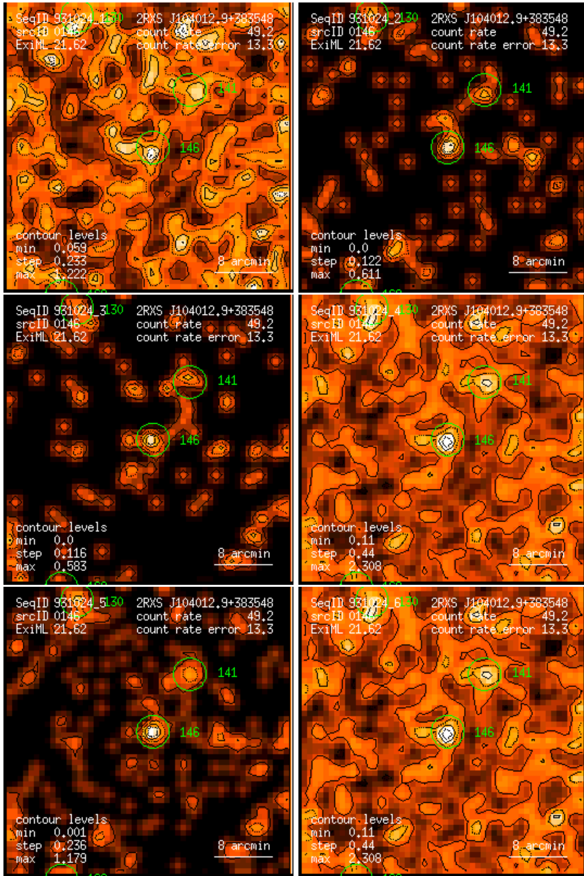
Figure 146: RASS 931024: detection 0146: band rate images, Gaussian filter: (1) PSPC channels 11 – 41, (2) 52 – 90, (3) 91 – 201, (4) 11 – 235, (5) 52 – 201, (6) 11 – 201. Broad band rates in counts/ks. Band rate contour levels in counts/ks/arcmin 2 .
