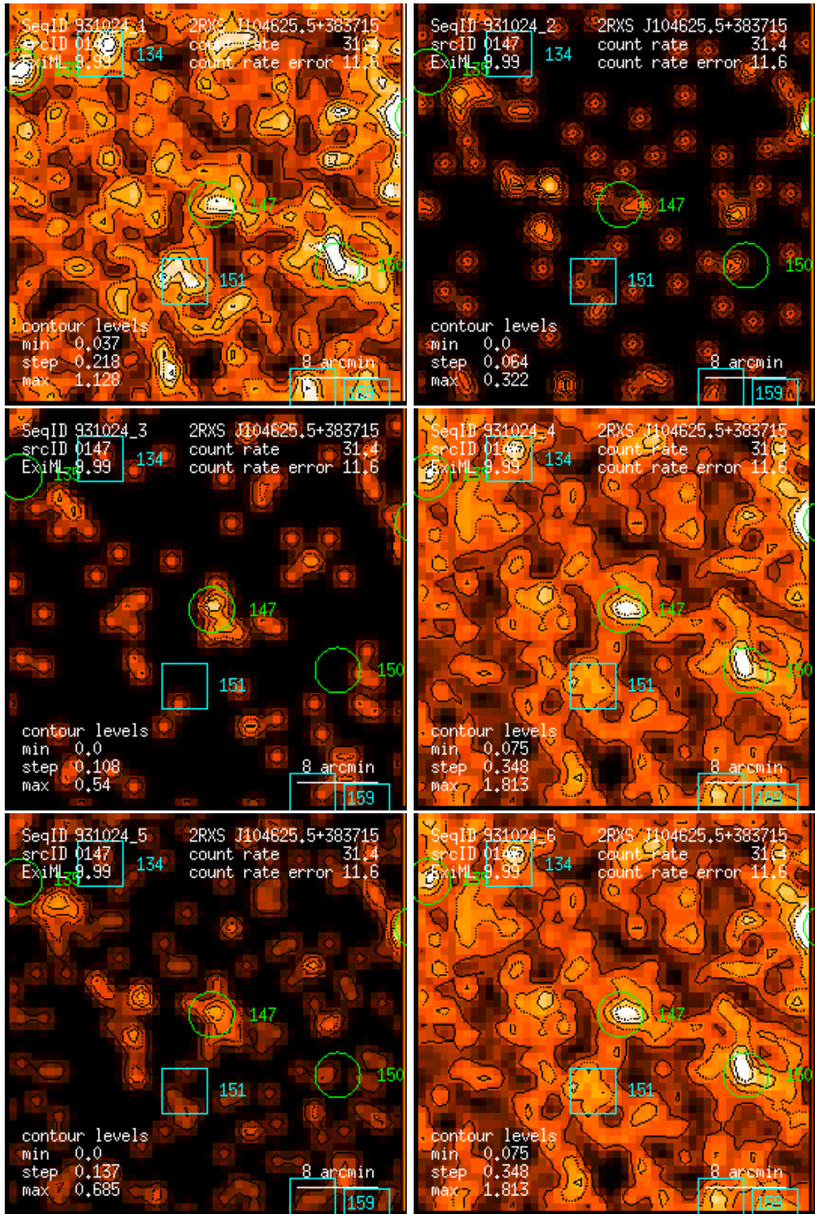
Figure 147: RASS 931024: detection 0147: band rate images, Gaussian filter: (1) PSPC channels 11 – 41, (2) 52 – 90, (3) 91 – 201, (4) 11 – 235, (5) 52 – 201, (6) 11 – 201. Broad band rates in counts/ks. Band rate contour levels in counts/ks/arcmin 2 .
