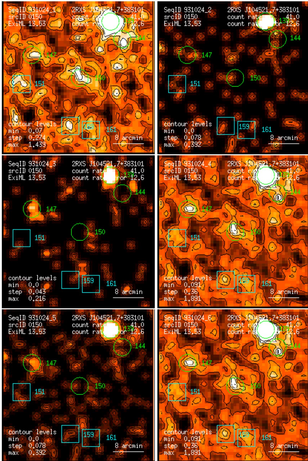
Figure 150: RASS 931024: detection 0150: band rate images, Gaussian filter: (1) PSPC channels 11 – 41, (2) 52 – 90, (3) 91 – 201, (4) 11 – 235, (5) 52 – 201, (6) 11 – 201. Broad band rates in counts/ks. Band rate contour levels in counts/ks/arcmin 2 .
