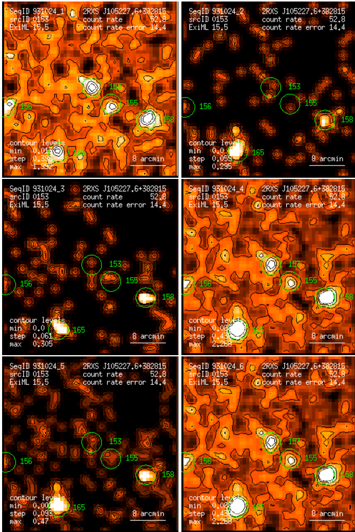
Figure 153: RASS 931024: detection 0153: band rate images, Gaussian filter: (1) PSPC channels 11 – 41, (2) 52 – 90, (3) 91 – 201, (4) 11 – 235, (5) 52 – 201, (6) 11 – 201. Broad band rates in counts/ks. Band rate contour levels in counts/ks/arcmin 2 .
