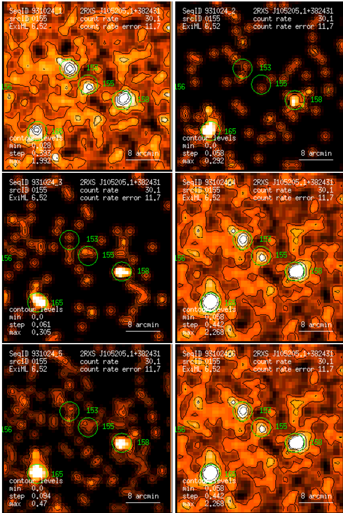
Figure 155: RASS 931024: detection 0155: band rate images, Gaussian filter: (1) PSPC channels 11 – 41, (2) 52 – 90, (3) 91 – 201, (4) 11 – 235, (5) 52 – 201, (6) 11 – 201. Broad band rates in counts/ks. Band rate contour levels in counts/ks/arcmin 2 .
