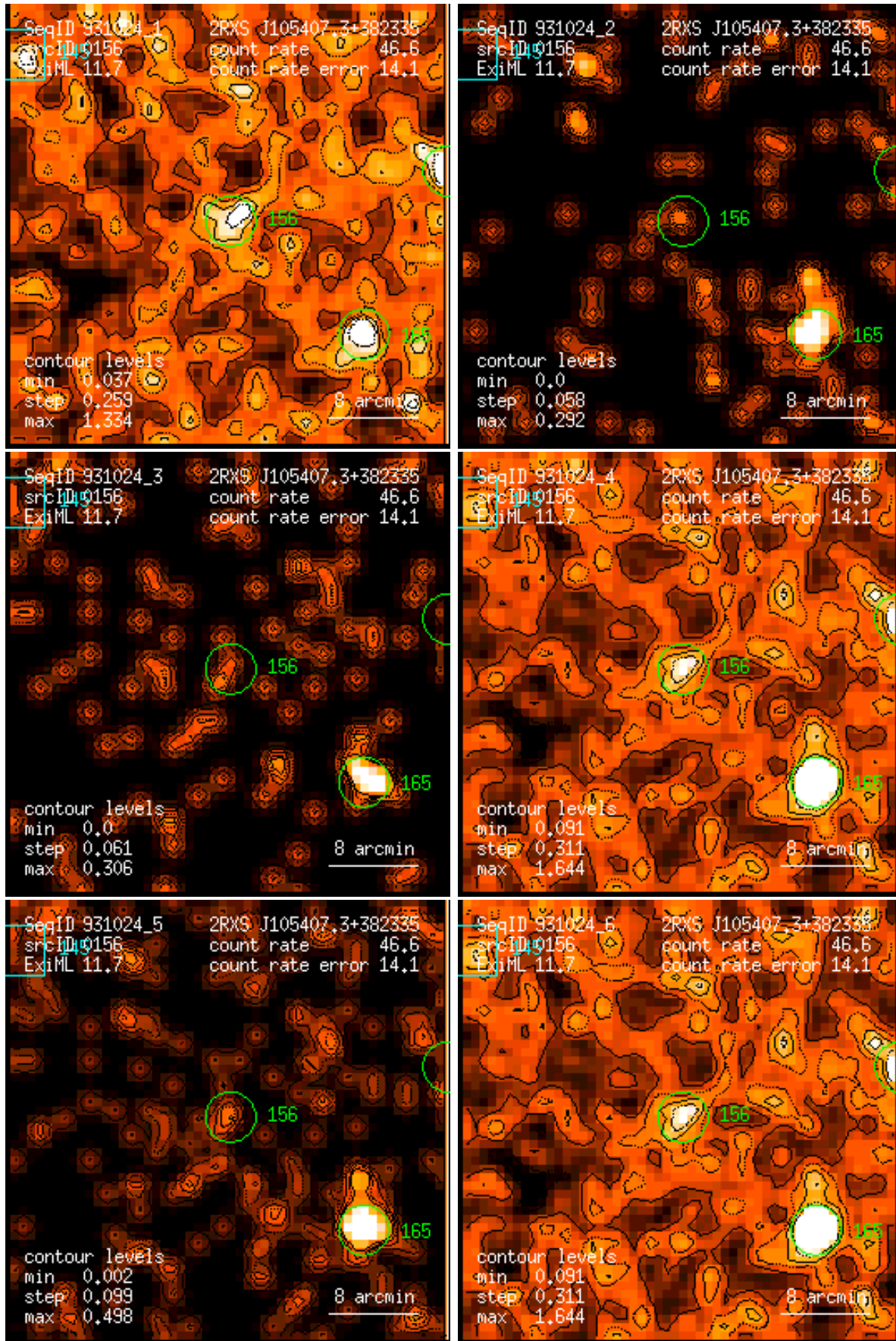
Figure 156: RASS 931024: detection 0156: band rate images, Gaussian filter: (1) PSPC channels 11 – 41, (2) 52 – 90, (3) 91 – 201, (4) 11 – 235, (5) 52 – 201, (6) 11 – 201. Broad band rates in counts/ks. Band rate contour levels in counts/ks/arcmin 2 .
