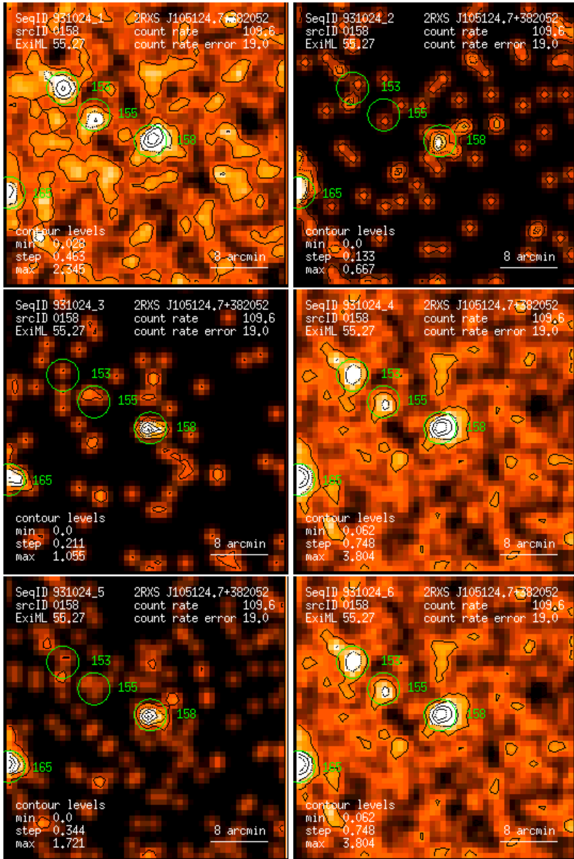
Figure 158: RASS 931024: detection 0158: band rate images, Gaussian filter: (1) PSPC channels 11 – 41, (2) 52 – 90, (3) 91 – 201, (4) 11 – 235, (5) 52 – 201, (6) 11 – 201. Broad band rates in counts/ks. Band rate contour levels in counts/ks/arcmin 2 .
