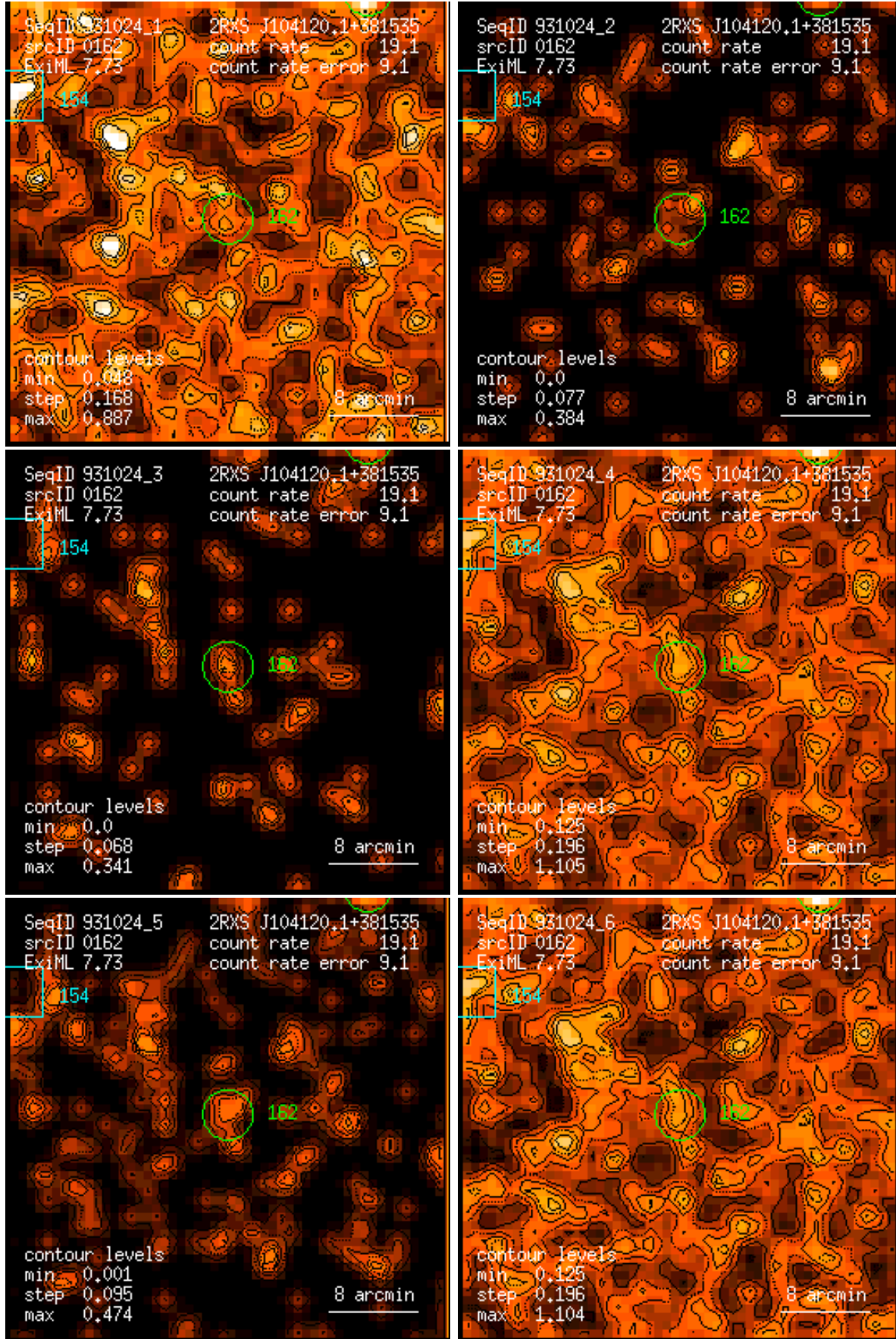
Figure 162: RASS 931024: detection 0162: band rate images, Gaussian filter: (1) PSPC channels 11 – 41, (2) 52 – 90, (3) 91 – 201, (4) 11 – 235, (5) 52 – 201, (6) 11 – 201. Broad band rates in counts/ks. Band rate contour levels in counts/ks/arcmin 2 .
