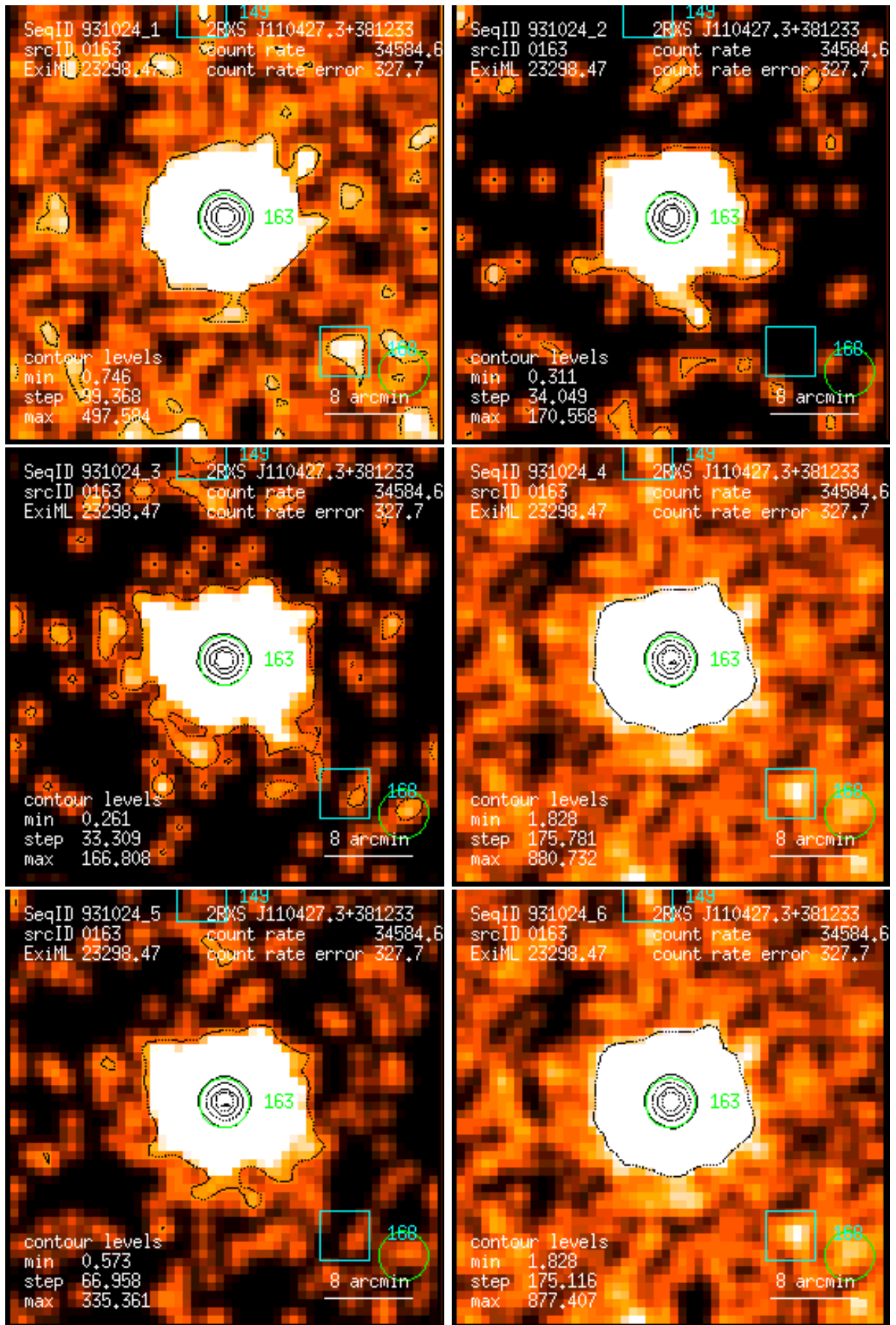
Figure 163: RASS 931024: detection 0163: band rate images, Gaussian filter: (1) PSPC channels 11 – 41, (2) 52 – 90, (3) 91 – 201, (4) 11 – 235, (5) 52 – 201, (6) 11 – 201. Broad band rates in counts/ks. Band rate contour levels in counts/ks/arcmin 2 .
