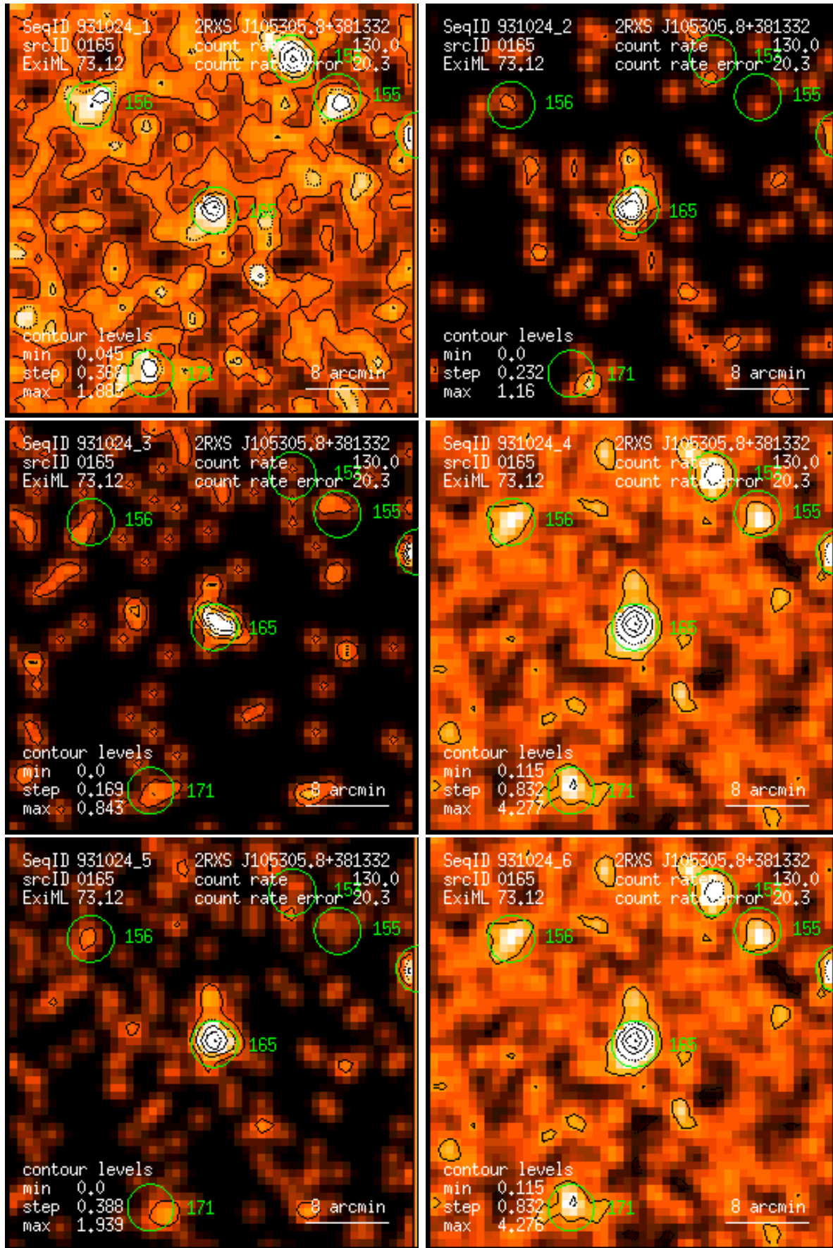
Figure 165: RASS 931024: detection 0165: band rate images, Gaussian filter: (1) PSPC channels 11 – 41, (2) 52 – 90, (3) 91 – 201, (4) 11 – 235, (5) 52 – 201, (6) 11 – 201. Broad band rates in counts/ks. Band rate contour levels in counts/ks/arcmin 2 .
