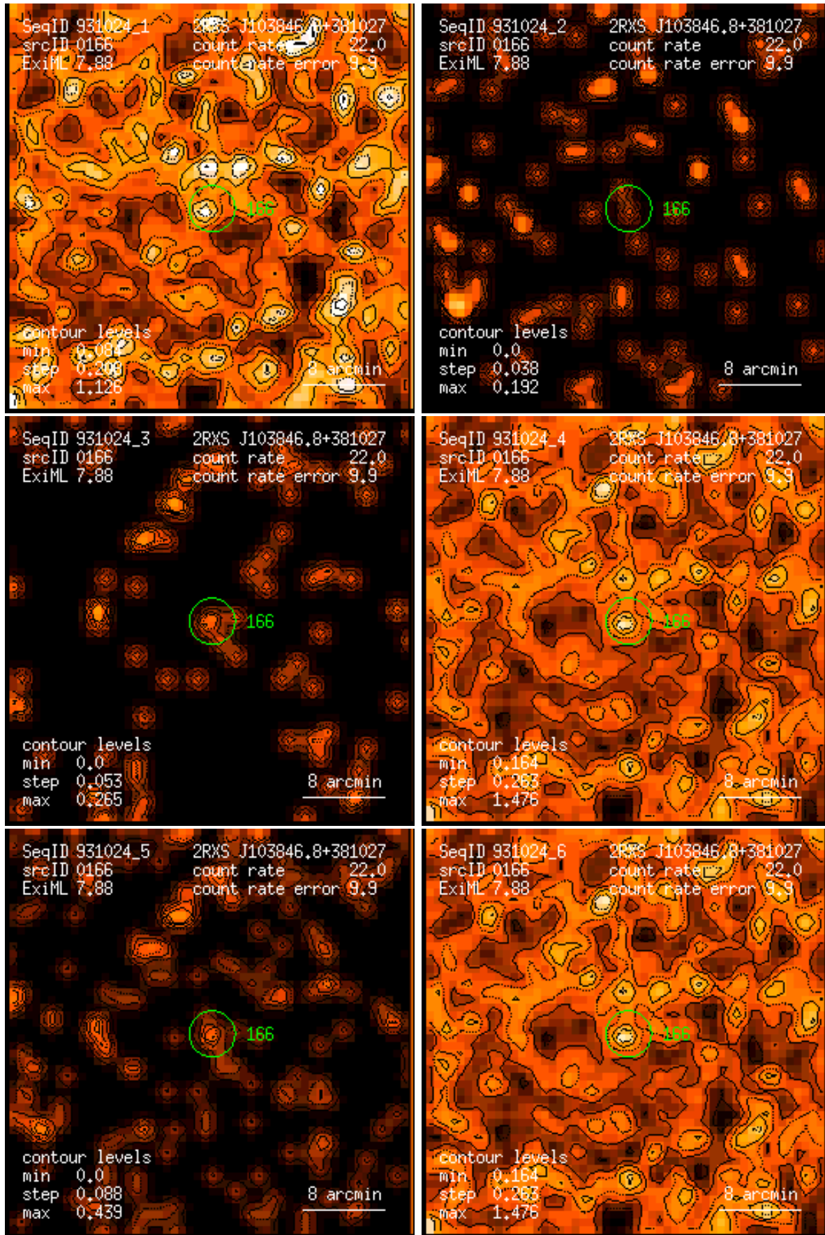
Figure 166: RASS 931024: detection 0166: band rate images, Gaussian filter: (1) PSPC channels 11 – 41, (2) 52 – 90, (3) 91 – 201, (4) 11 – 235, (5) 52 – 201, (6) 11 – 201. Broad band rates in counts/ks. Band rate contour levels in counts/ks/arcmin 2 .
