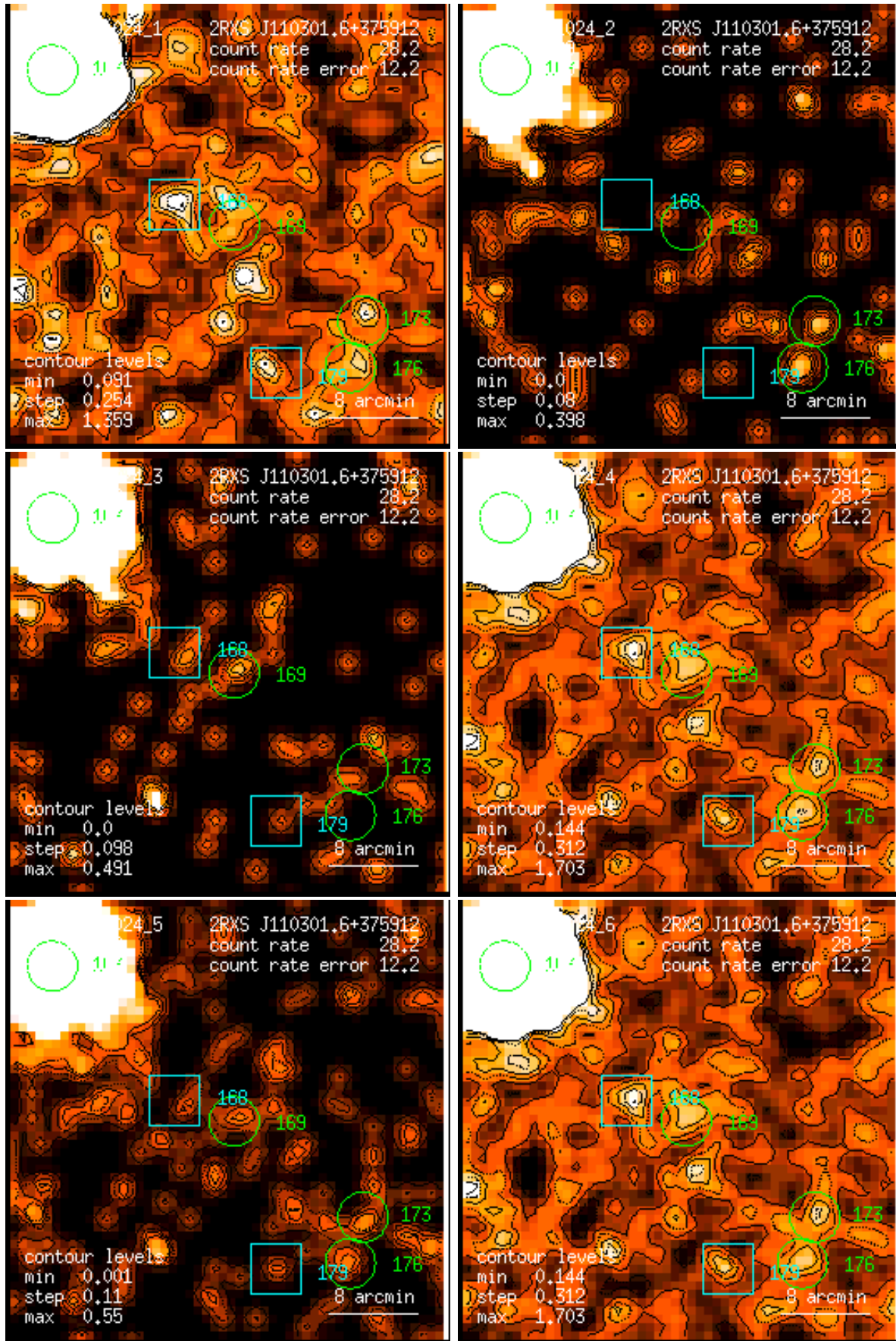
Figure 169: RASS 931024: detection 0169: band rate images, Gaussian filter: (1) PSPC channels 11 – 41, (2) 52 – 90, (3) 91 – 201, (4) 11 – 235, (5) 52 – 201, (6) 11 – 201. Broad band rates in counts/ks. Band rate contour levels in counts/ks/arcmin 2 .
