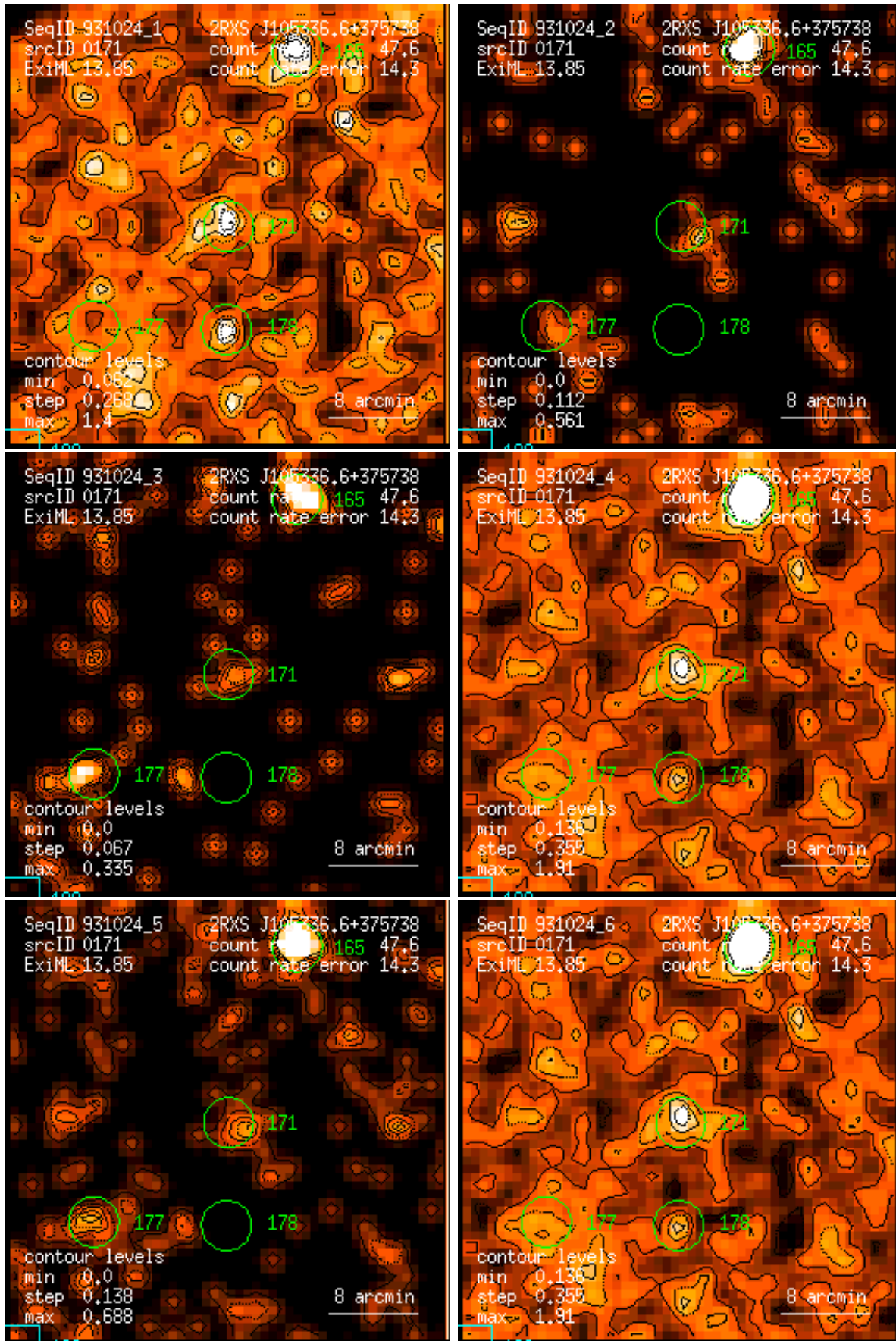
Figure 171: RASS 931024: detection 0171: band rate images, Gaussian filter: (1) PSPC channels 11 – 41, (2) 52 – 90, (3) 91 – 201, (4) 11 – 235, (5) 52 – 201, (6) 11 – 201. Broad band rates in counts/ks. Band rate contour levels in counts/ks/arcmin 2 .
