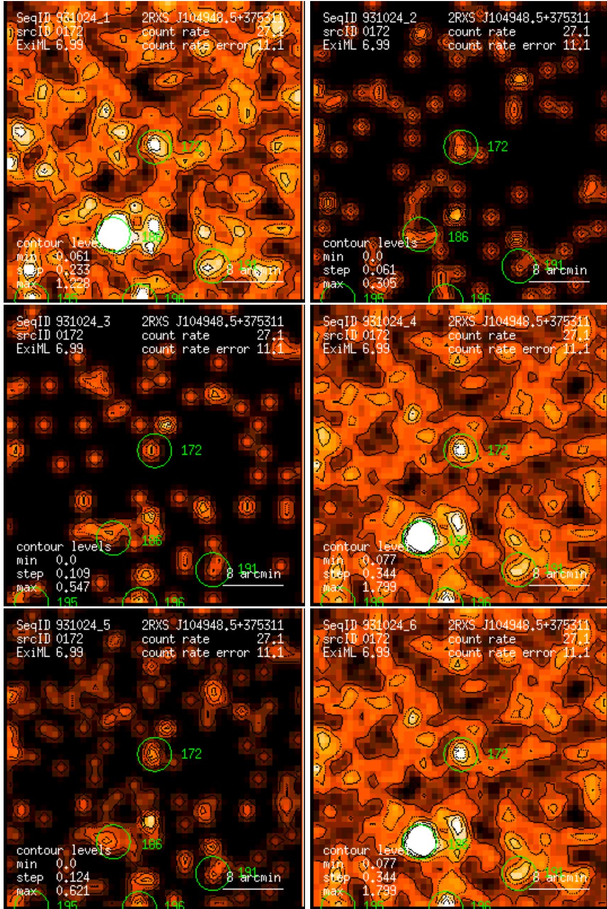
Figure 172: RASS 931024: detection 0172: band rate images, Gaussian filter: (1) PSPC channels 11 – 41, (2) 52 – 90, (3) 91 – 201, (4) 11 – 235, (5) 52 – 201, (6) 11 – 201. Broad band rates in counts/ks. Band rate contour levels in counts/ks/arcmin 2 .
