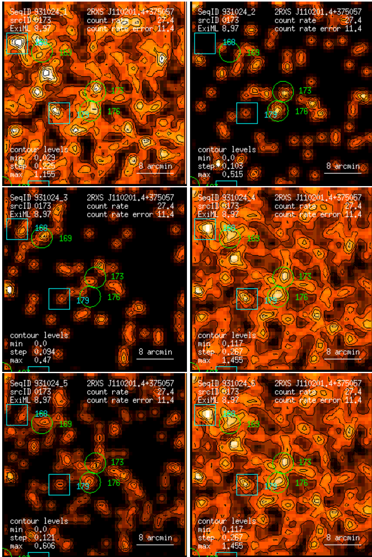
Figure 173: RASS 931024: detection 0173: band rate images, Gaussian filter: (1) PSPC channels 11 – 41, (2) 52 – 90, (3) 91 – 201, (4) 11 – 235, (5) 52 – 201, (6) 11 – 201. Broad band rates in counts/ks. Band rate contour levels in counts/ks/arcmin 2 .
