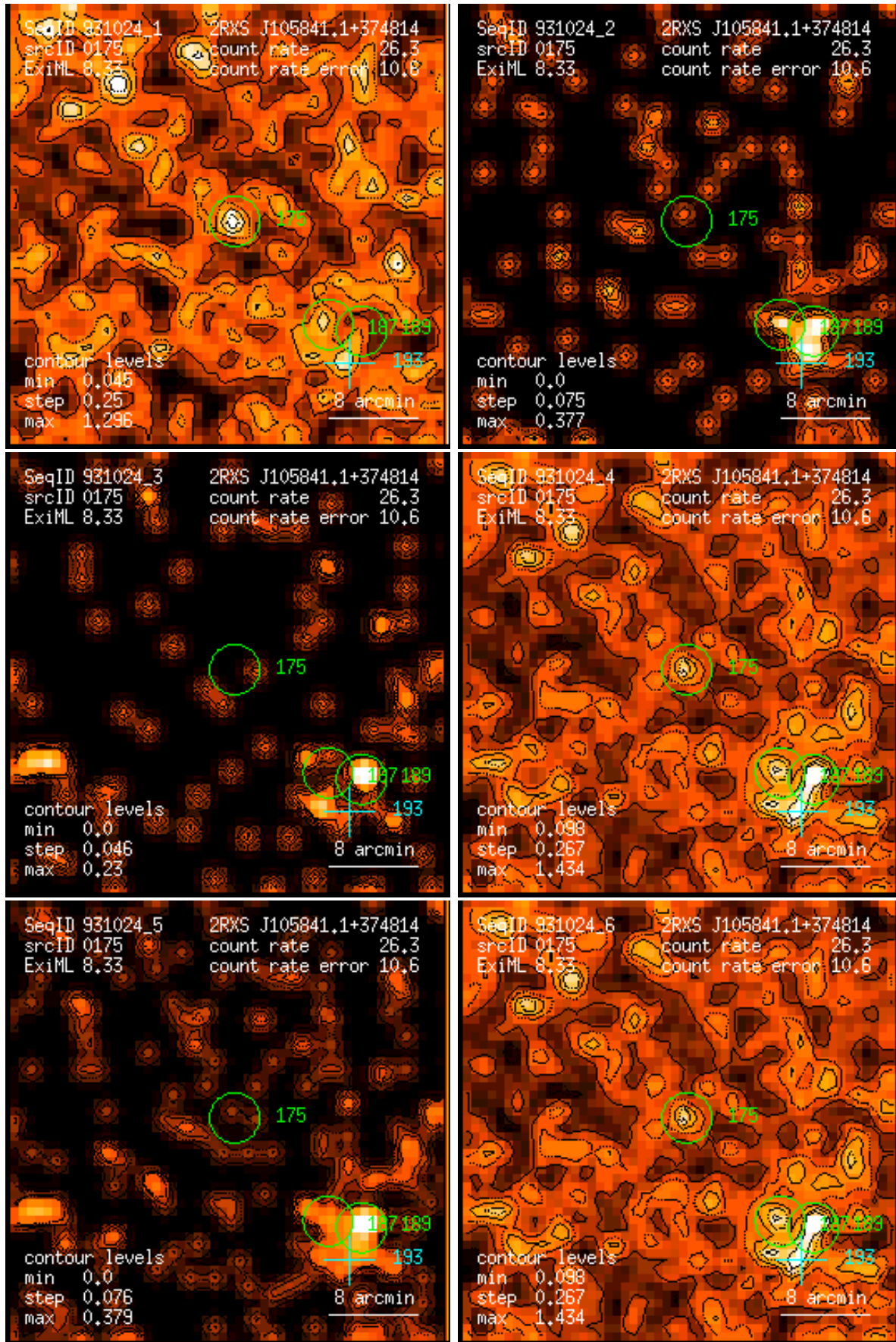
Figure 175: RASS 931024: detection 0175: band rate images, Gaussian filter: (1) PSPC channels 11 – 41, (2) 52 – 90, (3) 91 – 201, (4) 11 – 235, (5) 52 – 201, (6) 11 – 201. Broad band rates in counts/ks. Band rate contour levels in counts/ks/arcmin 2 .
