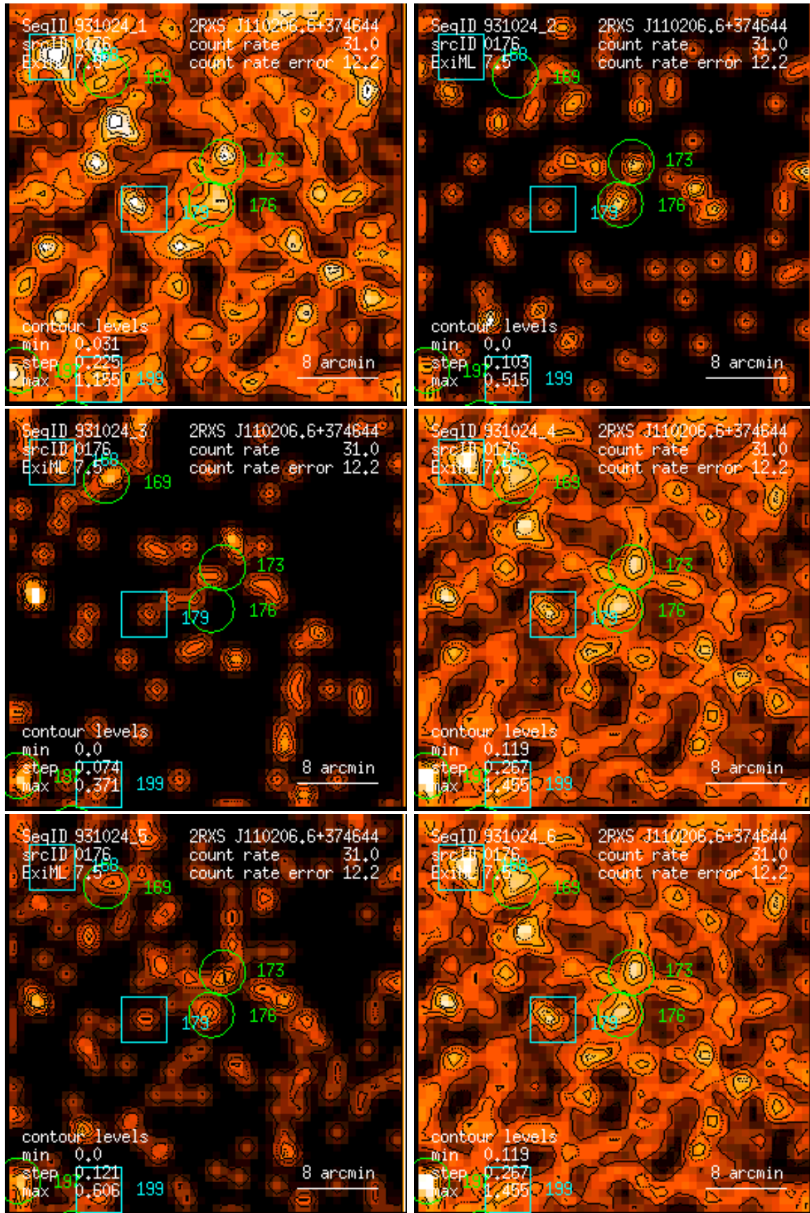
Figure 176: RASS 931024: detection 0176: band rate images, Gaussian filter: (1) PSPC channels 11 – 41, (2) 52 – 90, (3) 91 – 201, (4) 11 – 235, (5) 52 – 201, (6) 11 – 201. Broad band rates in counts/ks. Band rate contour levels in counts/ks/arcmin 2 .
