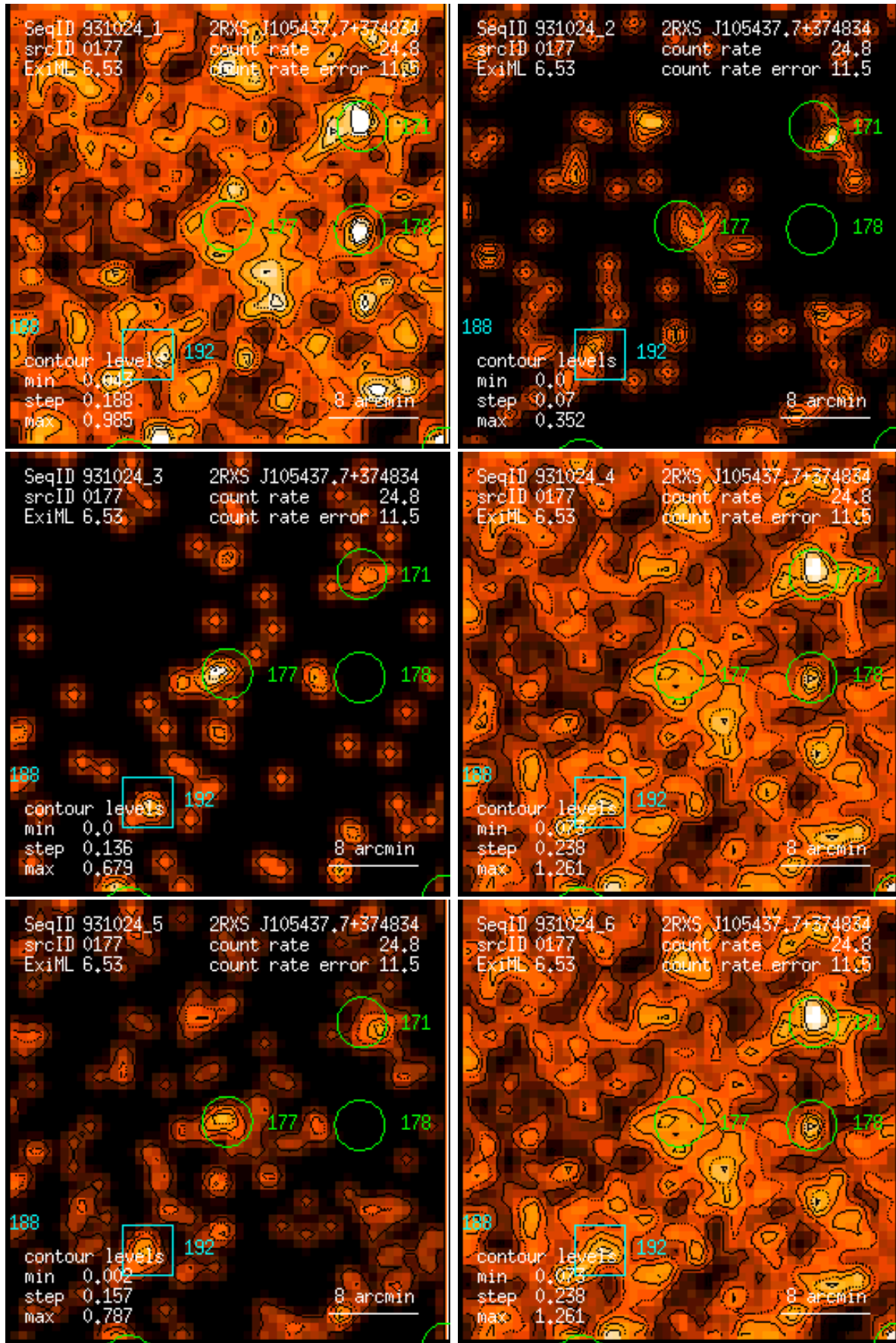
Figure 177: RASS 931024: detection 0177: band rate images, Gaussian filter: (1) PSPC channels 11 – 41, (2) 52 – 90, (3) 91 – 201, (4) 11 – 235, (5) 52 – 201, (6) 11 – 201. Broad band rates in counts/ks. Band rate contour levels in counts/ks/arcmin 2 .
