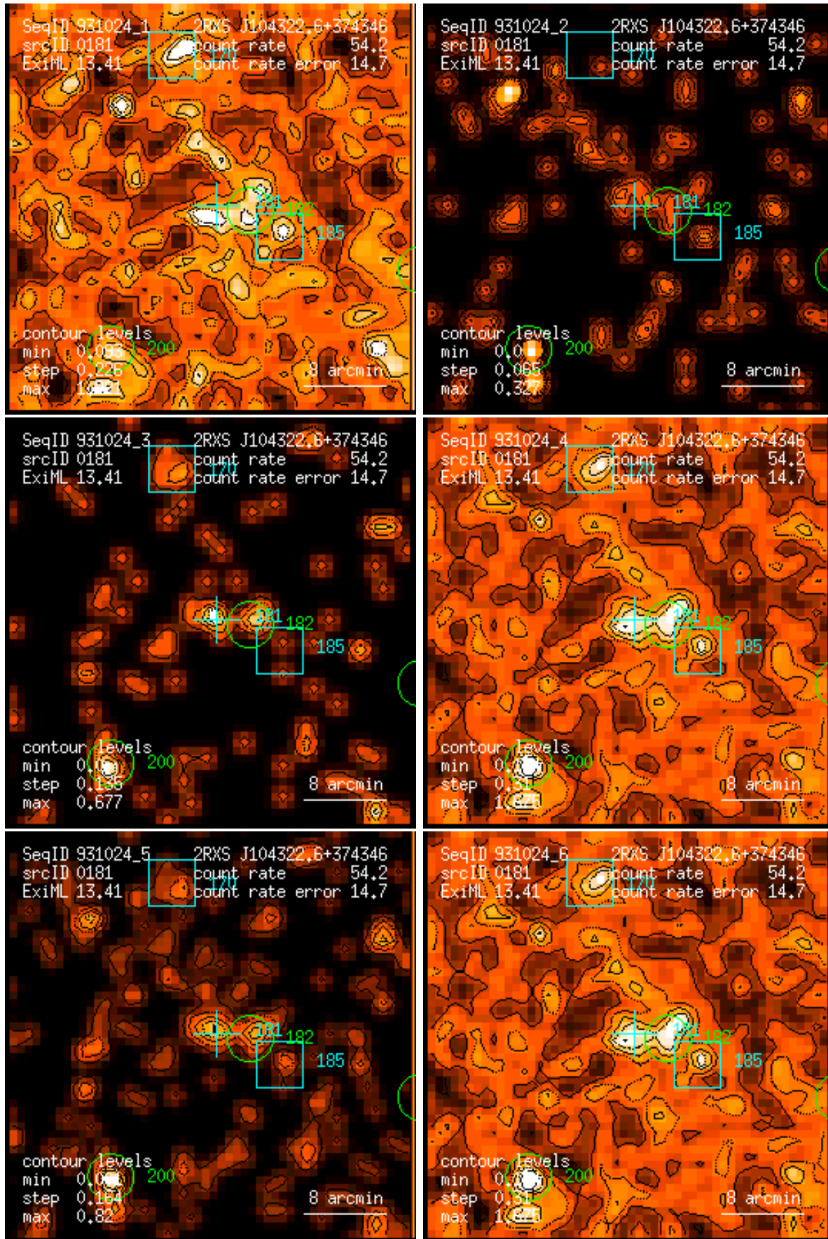
Figure 181: RASS 931024: detection 0181: band rate images, Gaussian filter: (1) PSPC channels 11 – 41, (2) 52 – 90, (3) 91 – 201, (4) 11 – 235, (5) 52 – 201, (6) 11 – 201. Broad band rates in counts/ks. Band rate contour levels in counts/ks/arcmin 2 .
