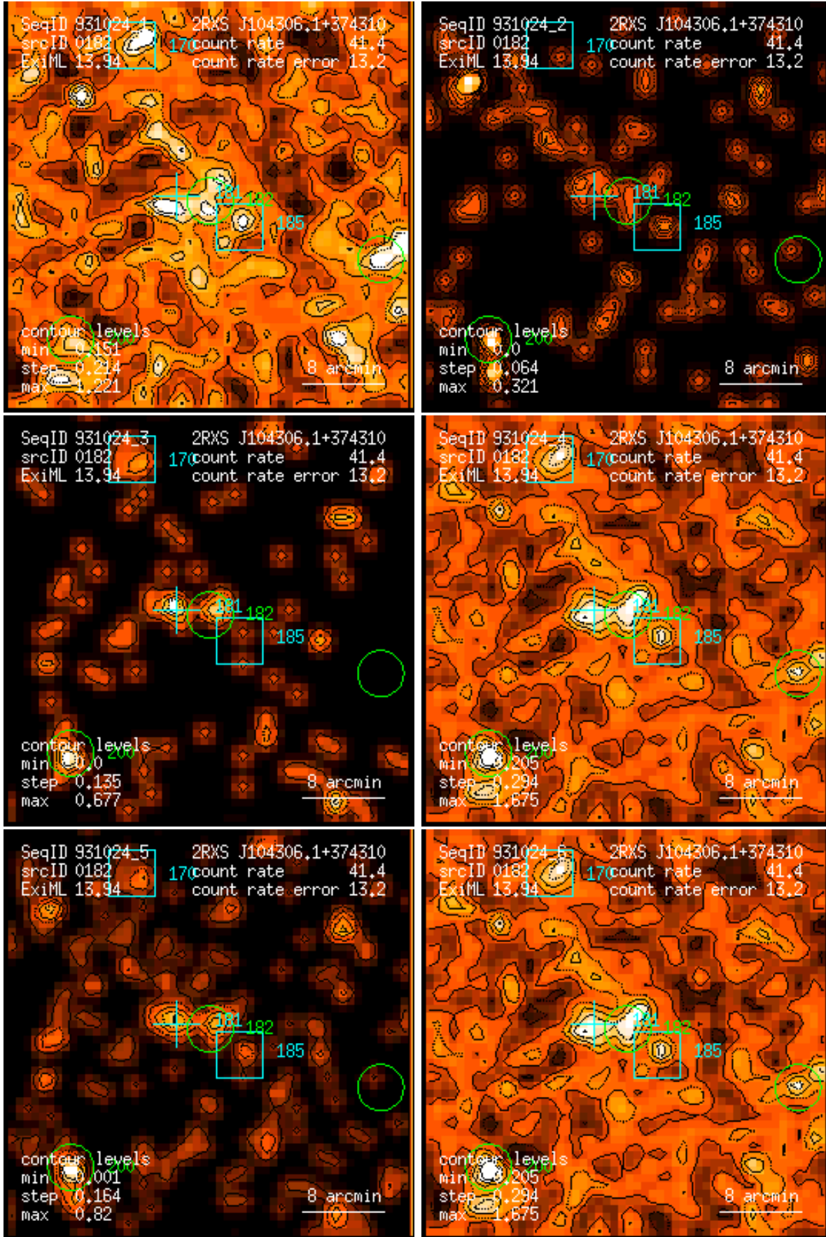
Figure 182: RASS 931024: detection 0182: band rate images, Gaussian filter: (1) PSPC channels 11 – 41, (2) 52 – 90, (3) 91 – 201, (4) 11 – 235, (5) 52 – 201, (6) 11 – 201. Broad band rates in counts/ks. Band rate contour levels in counts/ks/arcmin 2 .
