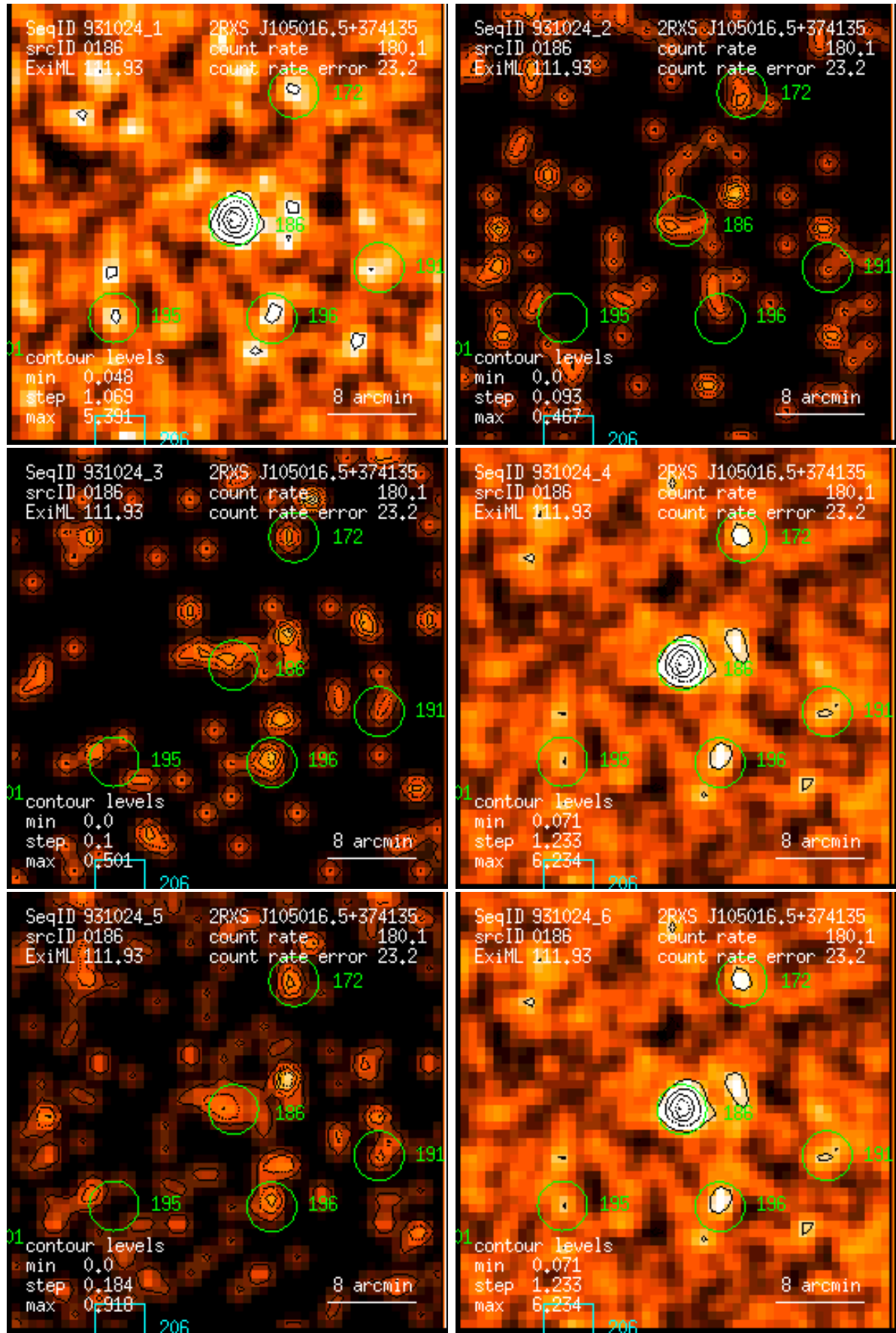
Figure 186: RASS 931024: detection 0186: band rate images, Gaussian filter: (1) PSPC channels 11 – 41, (2) 52 – 90, (3) 91 – 201, (4) 11 – 235, (5) 52 – 201, (6) 11 – 201. Broad band rates in counts/ks. Band rate contour levels in counts/ks/arcmin 2 .
