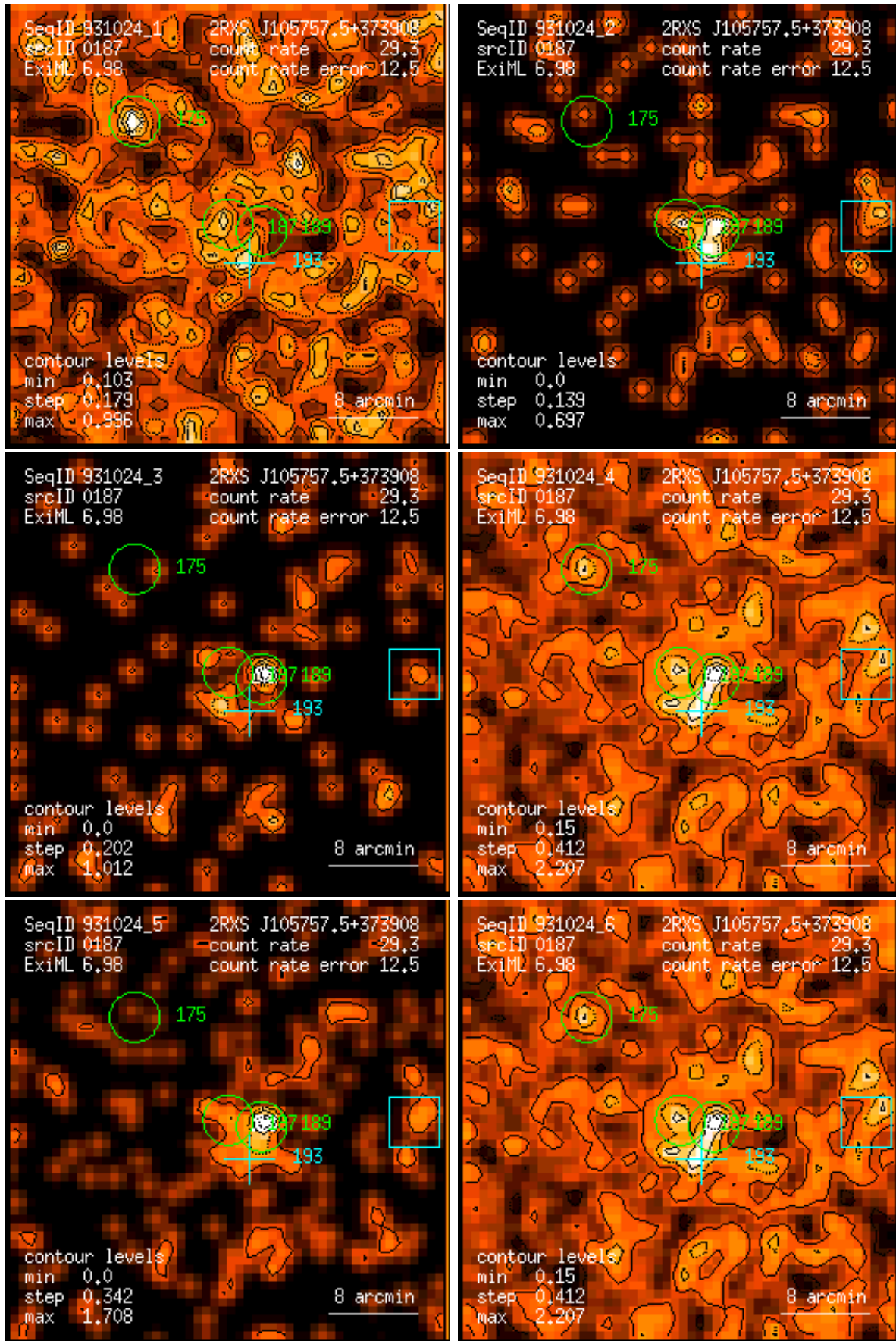
Figure 187: RASS 931024: detection 0187: band rate images, Gaussian filter: (1) PSPC channels 11 – 41, (2) 52 – 90, (3) 91 – 201, (4) 11 – 235, (5) 52 – 201, (6) 11 – 201. Broad band rates in counts/ks. Band rate contour levels in counts/ks/arcmin 2 .
