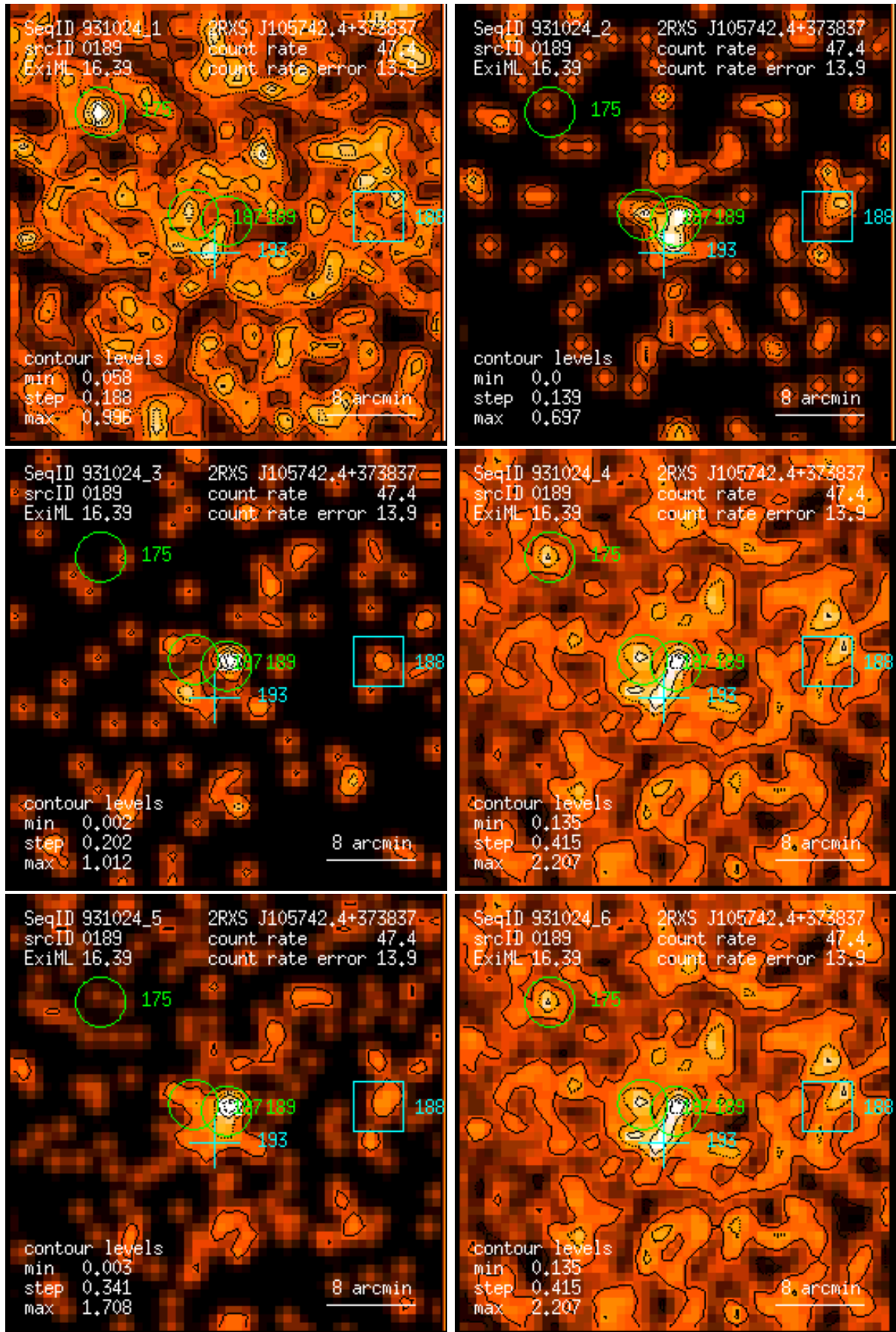
Figure 189: RASS 931024: detection 0189: band rate images, Gaussian filter: (1) PSPC channels 11 – 41, (2) 52 – 90, (3) 91 – 201, (4) 11 – 235, (5) 52 – 201, (6) 11 – 201. Broad band rates in counts/ks. Band rate contour levels in counts/ks/arcmin 2 .
